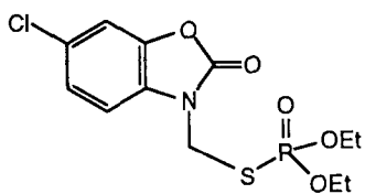
Fig. 1. Chemical structure of phosalone
