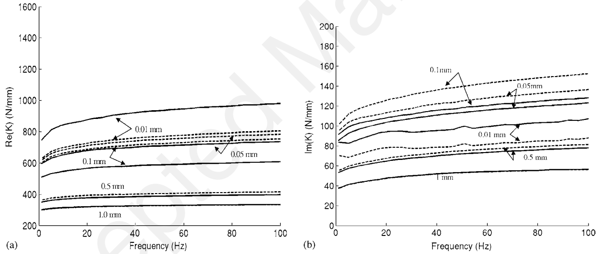
Fig. 15. Shear test and creep kernels. Measured (dashed line) and predicted (solid line) real (a) and imaginary (b) parts of the dynamic stiffness.
