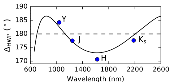
Fig. 7. HWP retardance as a function of wavelength as specified by the manufacturer 2 compared to the determined HWP retardance ( \Delta_{\text{HWP}} ) in the Y -, J -, H -, and K_s -band.
