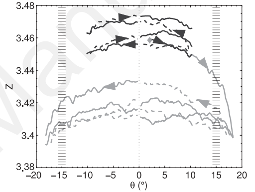
Figure 3. Coordination number of the grains as a function of the pile slope (same symbols as figure 1).
