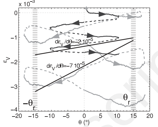
Figure 2. Estimation of the volumetric strain as a function of the pile slope (same symbols as figure 1).
