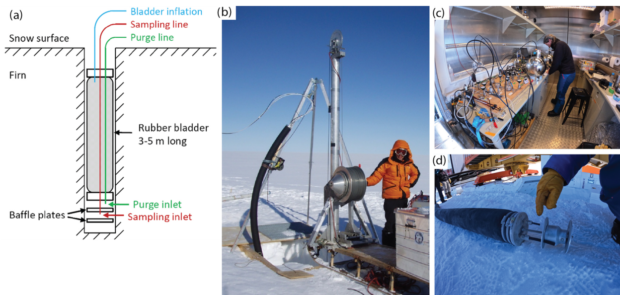
Figure 1. (a) Firn-air-pumping schematic courtesy of Christo Buizert, (b) sampling in the field photograph courtesy of Anne Solgaard, (c) sampling of the pumped air at Little Dome C, Antarctica 2022, and (d) the purge and sampling inlets on the actual setup. The same equipment was used for the firn air-pumping in Greenland in 2018.
