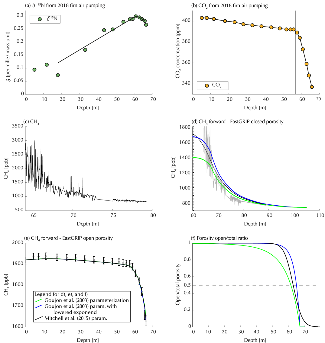
Figure 2. Measurements from the firn air-pumping campaign on the S6 borehole indicating that the transition of the diffusive to non-diffusive zone lies at around 61 m for (a) \delta^{15}\text{N} (not corrected for thermal fractionation) and 58 m depth for (b) \text{CO}_2 . (c) \text{CH}_4 measured in the ice core, as a function of depth, around the bubble close-off. (d) Forward modeling of \text{CH}_4 for closed porosity. (e) Laboratory measurements of \text{CH}_4 in the air from the open porosity of firn (symbols) compared with IGE-GIPSA (Institut des Géosciences de l'Environnement and Grenoble images parole signal automatique) firn model results obtained with the two open- / closed-porosity ratio parameterizations shown in panel (d) (the two model results are nearly superimposed). (f) Open- / closed-porosity parameterizations used in the IGE-GIPSA firn model. Blue is for the usual parameterization using Eq. (6) in Witrant et al. (2012); green is for the exponential factor is reduced from 7.6 to 3.0.
