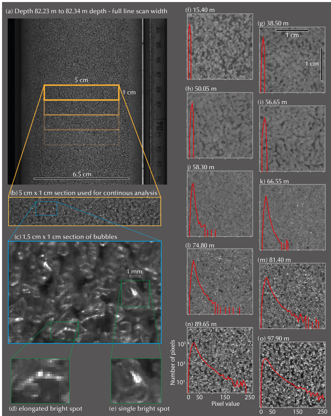
Figure 4. (a) An 11 cm section of a 165 cm long line scan image in its full width from 82.23 to 82.34 m depth. The 5 cm \times 1 cm sections used for the bright-spot and bubble analysis are indicated in yellow and in panel (b). (c) Close-up of the ice and bubble structure (1.5 cm \times 1 cm). (d) An elongated bright spot. Depending on the pixel value thresholding, this could be counted as one or multiple bright spots. (e) A single bright spot made up of many pixels. This is used as a proxy for counting bubbles. (f–o) Some 2 cm \times 2 cm example images across the upper 100 m, with the scale in panel (g). In red is the log-scale pixel distribution of image sections, with the scale in (n) and with the same scale for the images in panels (f) to (o). Note that all images have been brightness-enhanced for better visualization. Spots appearing bright to the eye have pixel values above 60.
