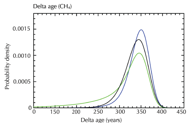
Figure 8. Delta age distributions using different parameterizations (see Fig. 2). The different parameterizations discussed throughout this paper all result in a delta age of around 350 years.
