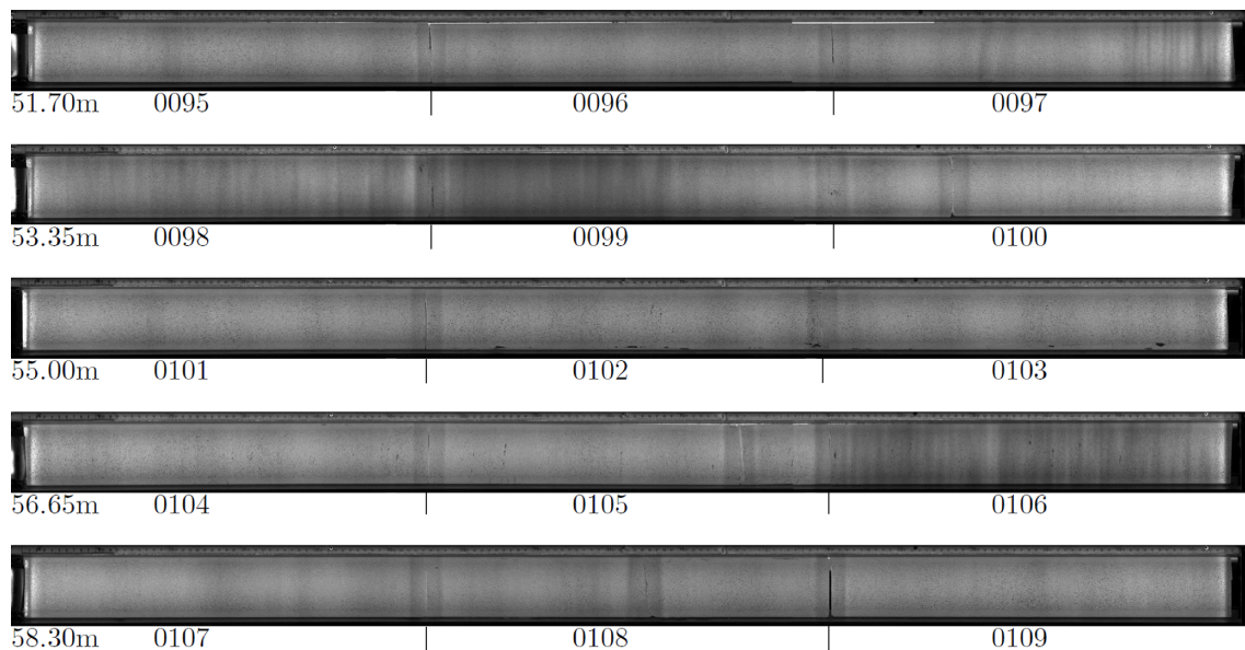
Figure D1. Bags 95 to 109 showing brightness variations in the line scan images and melt layers (from overview booklet; Westhoff et al., 2019).
