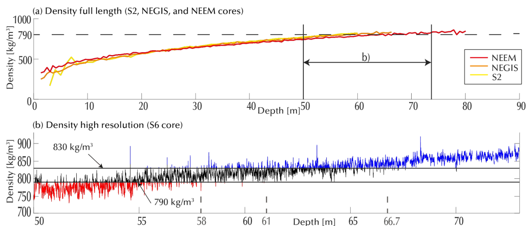
Figure 3. (a) Density of the S2, NEGIS, and NEEM ice cores as 1 m, 55 cm, and 55 cm averages, respectively, measured by weighing in the field. (b) High-resolution density of the S6 ice core derived from micro-CT measurements. Values below 790 \text{ kg m}^{-3} are in red, values above 830 \text{ kg m}^{-3} are in blue, and values in-between are in black. Depth results from Part I are in gray on the x axis.
