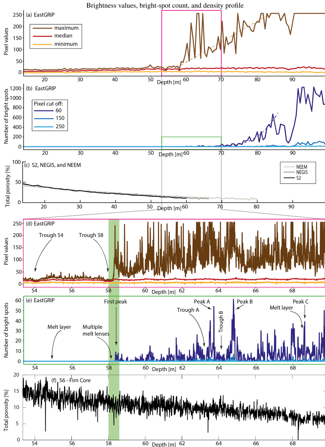
Figure 6. Depth of investigation from 13.75 to 99.40 m below the surface with one measurement every 55 cm (a, b). Detailed analysis from 53.35 to 69.85 m with continuous measurements every centimeter (d, e). Our analysis locates the OLID at 58.30 m depth. We find a linear increase in maximum values in panel (a) and a roughly exponential increase in bubbles in panel (b) (dashed lines). Both panels (d) and (e) show a sudden appearance of bright spots below 58.30 m, with the layering clearly visible in panel (e). (c) Total porosity calculated from density data of the S2, NEGIS, and NEEM ice cores and (f) total porosity from micro-CT density data of the S6 ice core (Freitag and Westhoff, 2024). The full high-resolution S6 profile will be published later.
