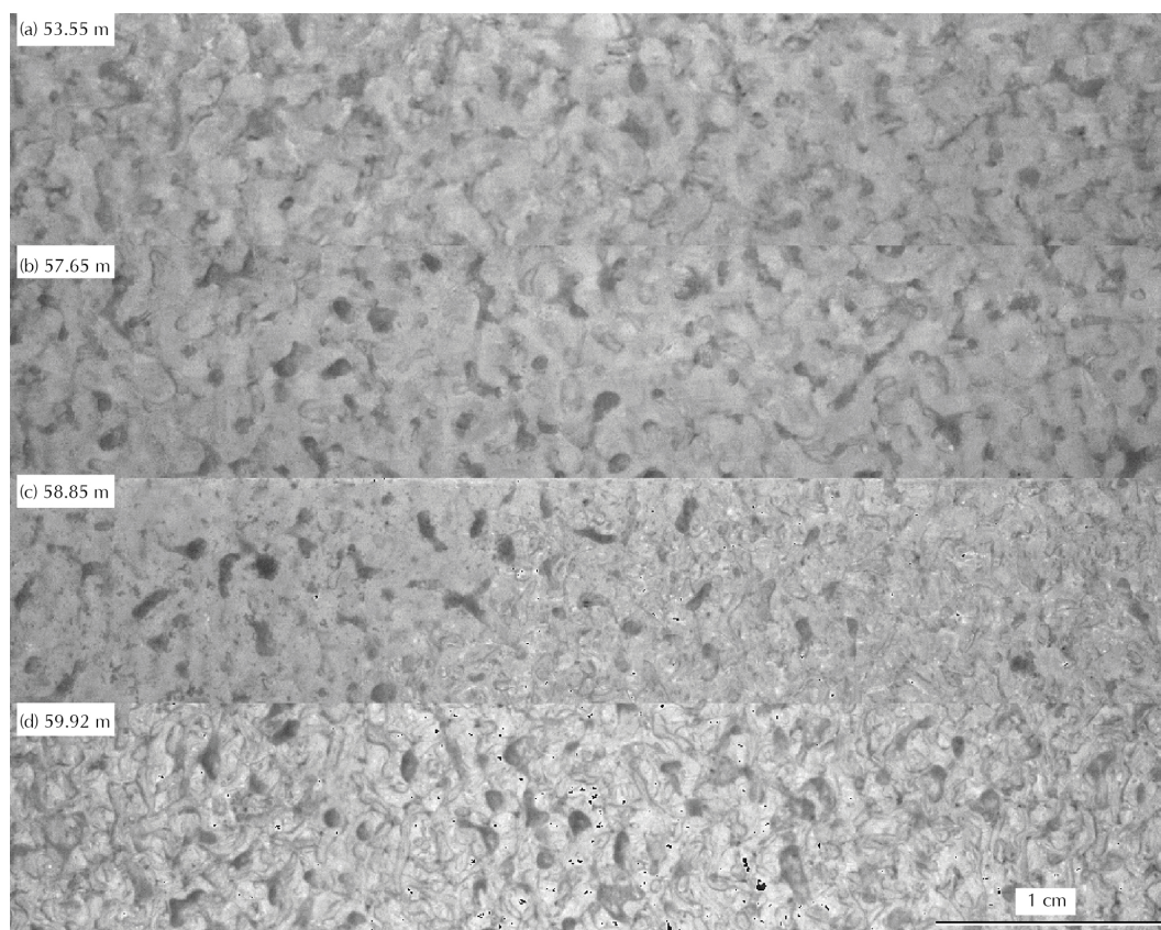
Figure C1. Brightness-enhanced images over the optical LID (EastGRIP). Panels (a) and (b) show the appearance of firn without bright spots (here converted to black). Panel (c) shows the transition, and panel (d) shows multiple bright spots and clearer firn–gas interfaces.
