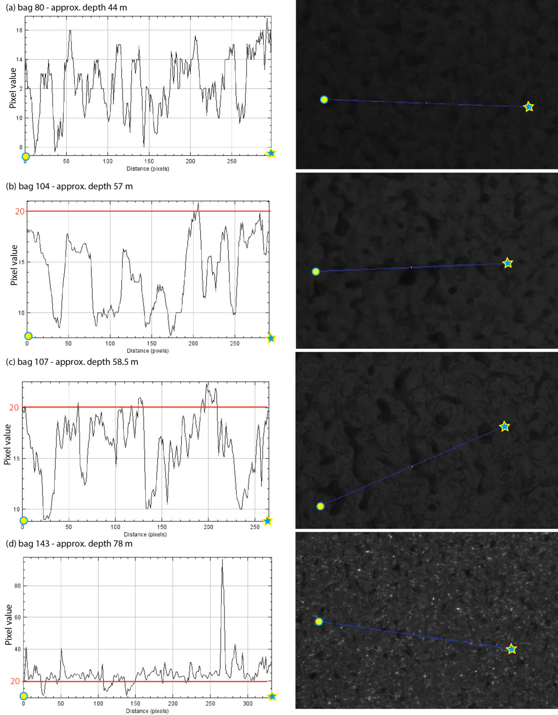
Figure B1. The change in the brightness appearance with depth. (a) Above the firm–ice transition, (b–c) the transition, and (d) below the firm–ice transition. The left-hand side shows the brightness profiles from the blue lines on the right-hand side. The image width is approximately 2 cm.
