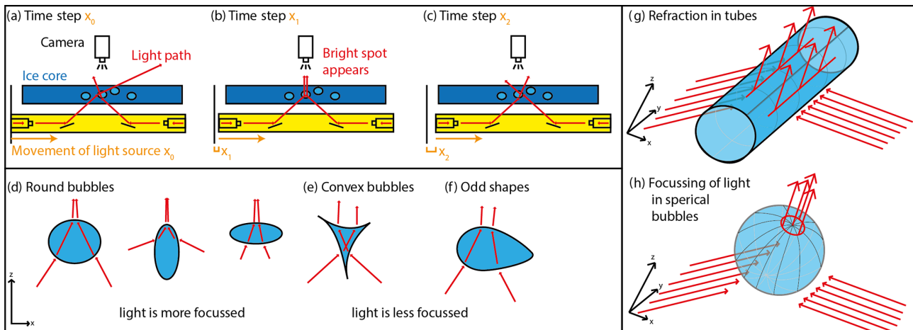
Figure 5. (a–c) Line scan setup with a fixed camera and ice core and a moving light source (yellow). In certain settings, the introduced light will refract and bundle, causing bright spots (b). The amount of light bundling is a geometric effect dependent on the bubble shape, e.g., (d) rounded bubbles, (e) convex bubbles, or (f) other shapes. The amount of bundling/focusing is also dependent on the 3D bubble shape as tubes bundle less often (g) than spheres (h).
