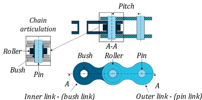
Fig. 1. Nomenclature of a modern roller chain.
