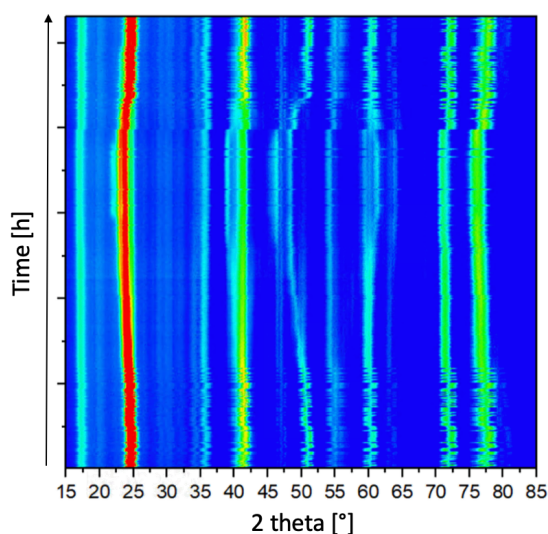
Figure 1. Contour plot representation of the neutron patterns collected during the operando experiment.
