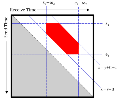
Figure 9: The support of the matrix ([s_1, e_1] : \omega_1)S_\alpha([s_2, e_2] : \omega_2) , where \Omega = \omega_1 + \omega_2
