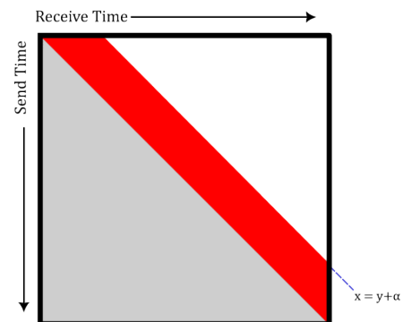
Figure 7: The support of the matrix S_{\alpha}
