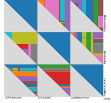
(d) A three by three slice of the fourth cumulant A^{(4)} .
