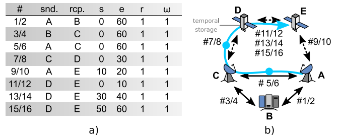
Figure 1: Example space network represented by a) a Contact plan table, and b) a static graph of the topology.
