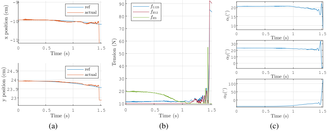
Figure 21: Time histories of (a) x and y , (b) f and (c) the \alpha_i for the trajectory from configuration 1 to 3 from with the CTC. For (b), the plot colors correspond to the cable colors in Fig. 17.
