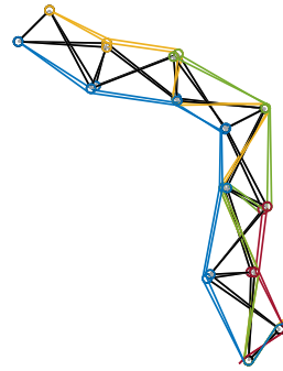
Figure 4: Robot configuration at f_{min} = 0 N and f_{min} = 1000 N for [x, y] = [-0.26, 0.36]^\top m and \gamma = \frac{\pi}{4} rad (springs not represented).
