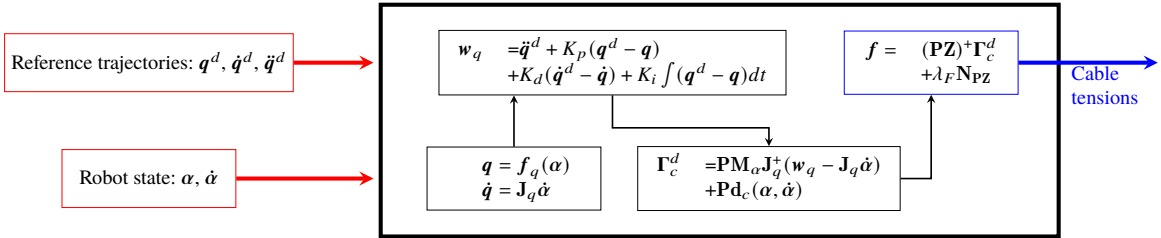
Figure 11: PCTC scheme
