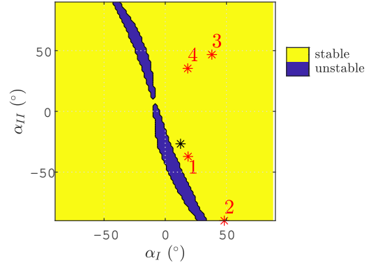
Figure 19: Stability domains of the control of \mathbf{q} = [x, y]^T for a robot with 3 joints and 3 cables under gravity and with the prototype springs in the joint space for the PCTC. The red stars corresponds to the numbered robot configurations of Fig. 17. The black star is the configuration at rest.
