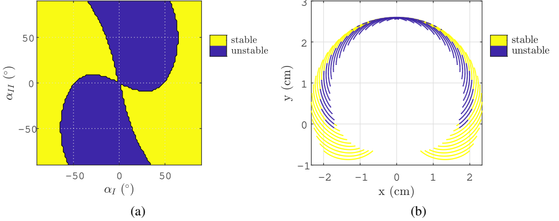
Figure 9: Stability domains of the control of \mathbf{q} = [x, y]^\top for a robot with 3 joints and 3 cables (a) in the joint space and (b) in the controlled variables space for the CTC
