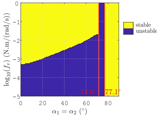
Figure 12: Stability domains of the control of \mathbf{q} = x for a robot with 2 joints and 2 cables against the robot joint angle and the viscous friction constant for the PCTC
