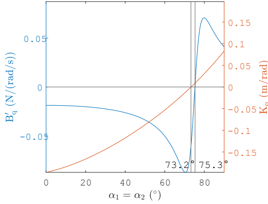
Figure 13: Plot of B'_q and K_q for \mathbf{q} = x against the joint angle for a robot with 2 joints and 2 cables
