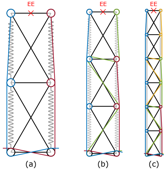
Figure 2: The three underactuated robots under study. (a) has 2 joints and 2 cables, (b) has 3 joints and 3 cables and (c) has 6 joints and 4 cables.
