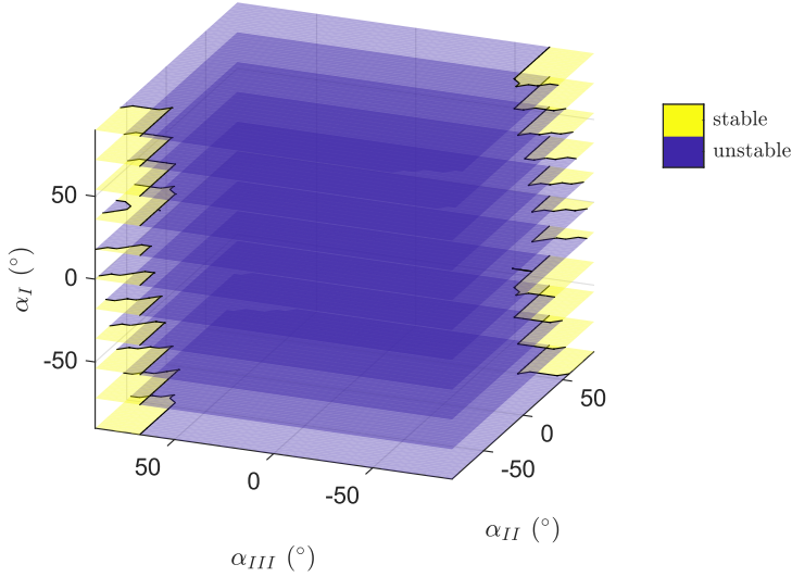
Figure 10: Stability domains of the control of \mathbf{q} = [x, y, \gamma]^\top for a robot with 6 joints and 4 cables in the joint space for the CTC
