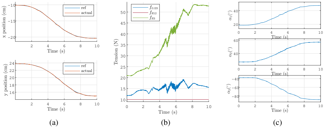
Figure 22: Time histories of (a) x and y , (b) f and (c) the \alpha_i for the trajectory from configuration 1 to 2 from with the PCTC. For (b), the plot colors correspond to the cable colors in Fig. 17.
