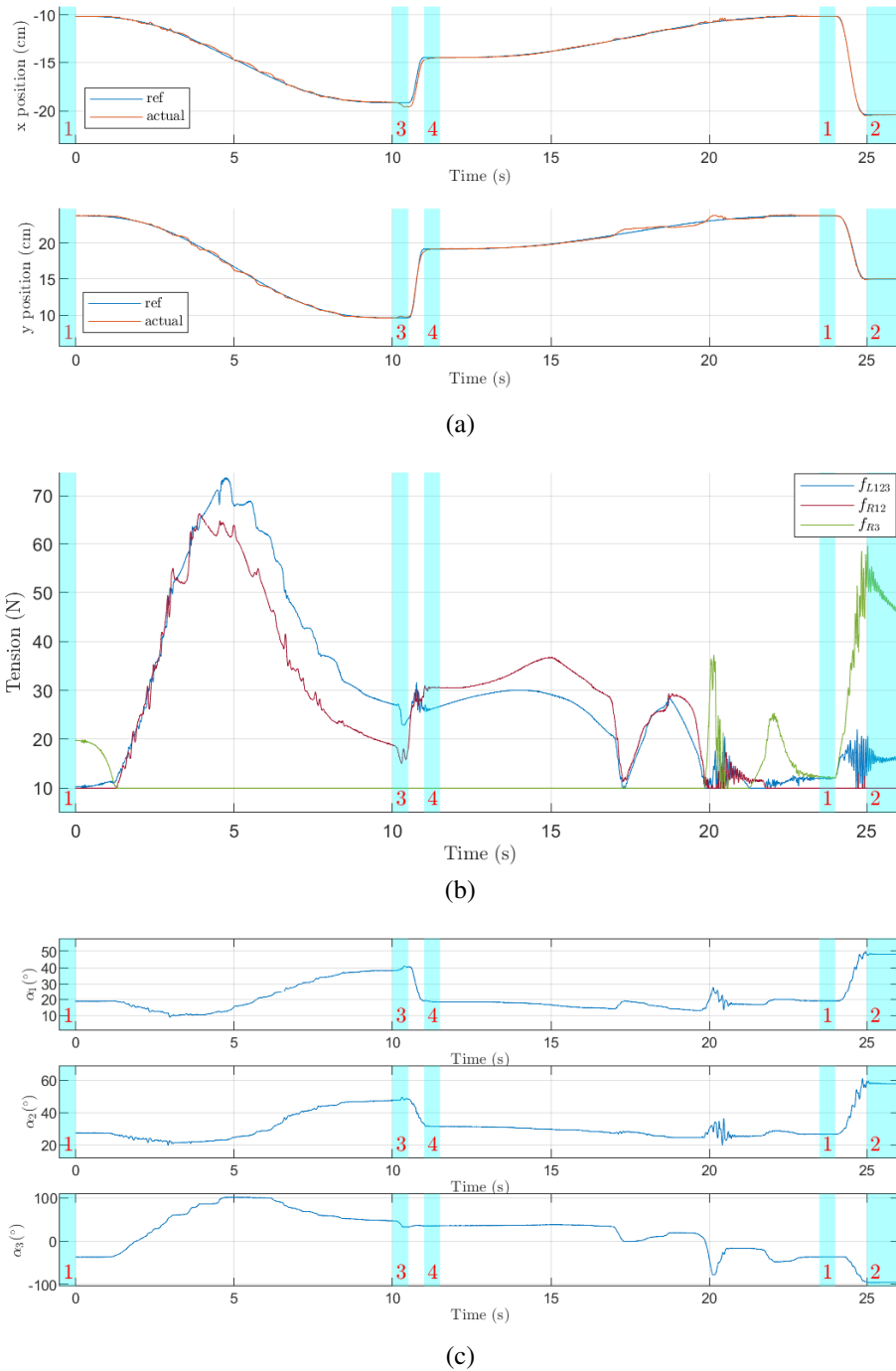
Figure 23: Time histories of (a) x and y , (b) f and (c) the \alpha_i for the trajectory from configuration 1 to 3, then to 4, then to 1, and finally to 2 with the PCTC. For (b), the plot colors correspond to the cable colors in Fig. 17. The light blue areas indicate the desired numbered robot configurations of Fig. 17
