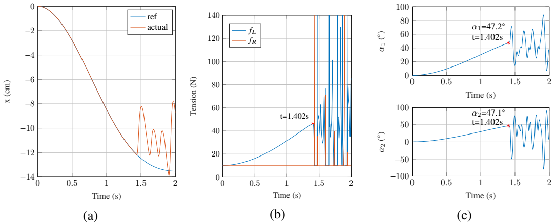
Figure 8: Simulation of the control of q = x for a robot with 2 joints and 2 cables with the CTC. (a) corresponds to the tracking of x over time, (b) illustrates the evolution of cable tension over time, and (c) shows the evolution of joint angles over time.
