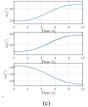
Figure 20: Time histories of (a) x and y , (b) \mathbf{f} and (c) the \alpha_i for the trajectory from configuration 1 to 2 from with the CTC. For (b), the plot colors correspond to the cable colors in Fig. 17.
