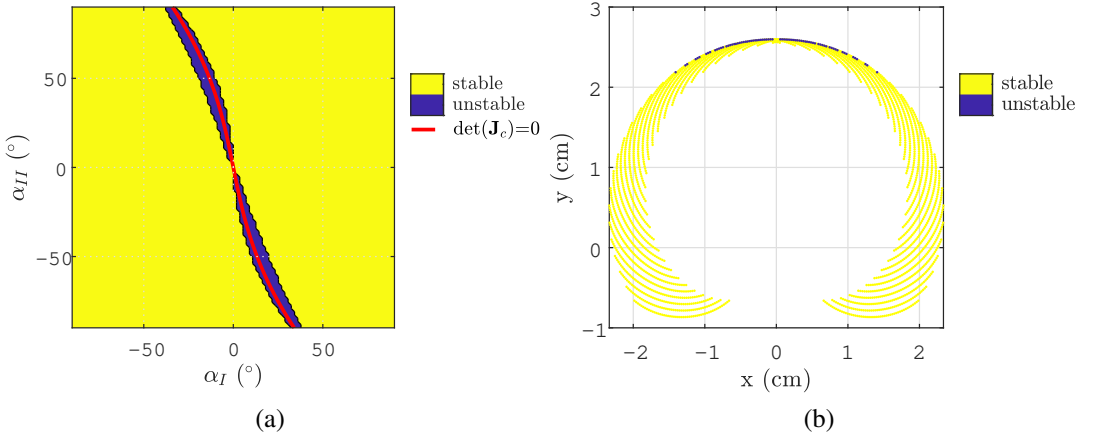
Figure 14: Stability domains of the control of \mathbf{q} = [x, y]^T for a robot with 3 joints and 3 cables (a) in the joint space and (b) in the controlled variables space for the PCTC
