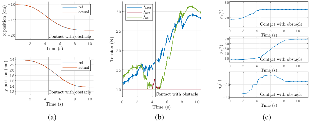
Figure 26: Time histories of (a) x and y , (b) \mathbf{f} and (c) the \alpha_i for the trajectory from configuration 1 to 5 using the PCTC. For (b), the plot colors correspond to the cable colors in Fig. 17. The vertical black line indicates when the robot enters in contact with the obstacle.
