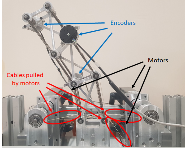
Figure 16: Prototype
