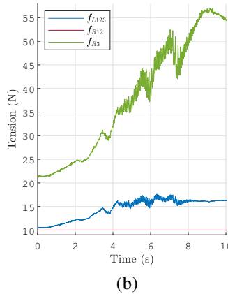
Figure 20: Time histories of (a) x and y , (b) \mathbf{f} and (c) the \alpha_i for the trajectory from configuration 1 to 2 from with the CTC. For (b), the plot colors correspond to the cable colors in Fig. 17.
