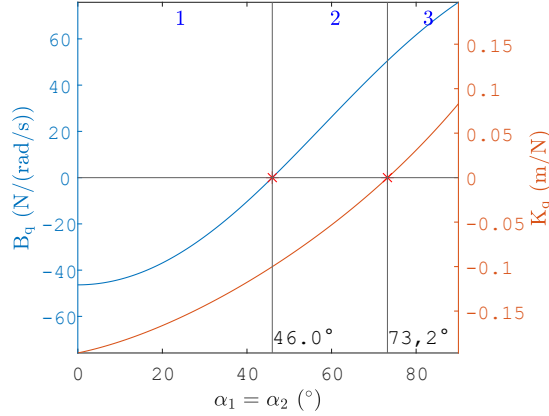
Figure 7: Plots of B_q and K_q for q = x against the joint angle for a robot with 2 joints and 2 cables
