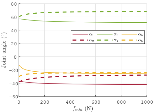
Figure 3: Joint angle evolution as a function of the lowest cable tension f_{min} for [x, y] = [-0.26, 0.36]^\top m and \gamma = \frac{\pi}{4} rad. The angles represented with the same color belong to the same metamodule. Continuous lines correspond to the first joint of the metamodule, while dashed lines represent the second joint of the metamodule.
