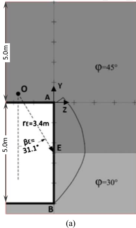
Fig. 7. Case of a tunnel driven in a two-layers frictional medium (a) cross-section of the critical failure mechanism (in the central vertical plane) as obtained from the analytical model (where \sigma_c = 9.1 kPa, \beta_E = 31.1^\circ , r_E = 3.4 m) and (b) and (c) two 3D views of the mechanism.
