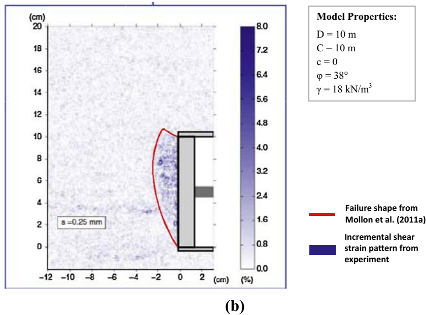
Fig. 2. Comparison of failure shape obtained from the analytical model by Mollon et al. (2011a) with the shape from experimental tests (a) by Berthoz (2012); (b) by Kirsch (2010).
