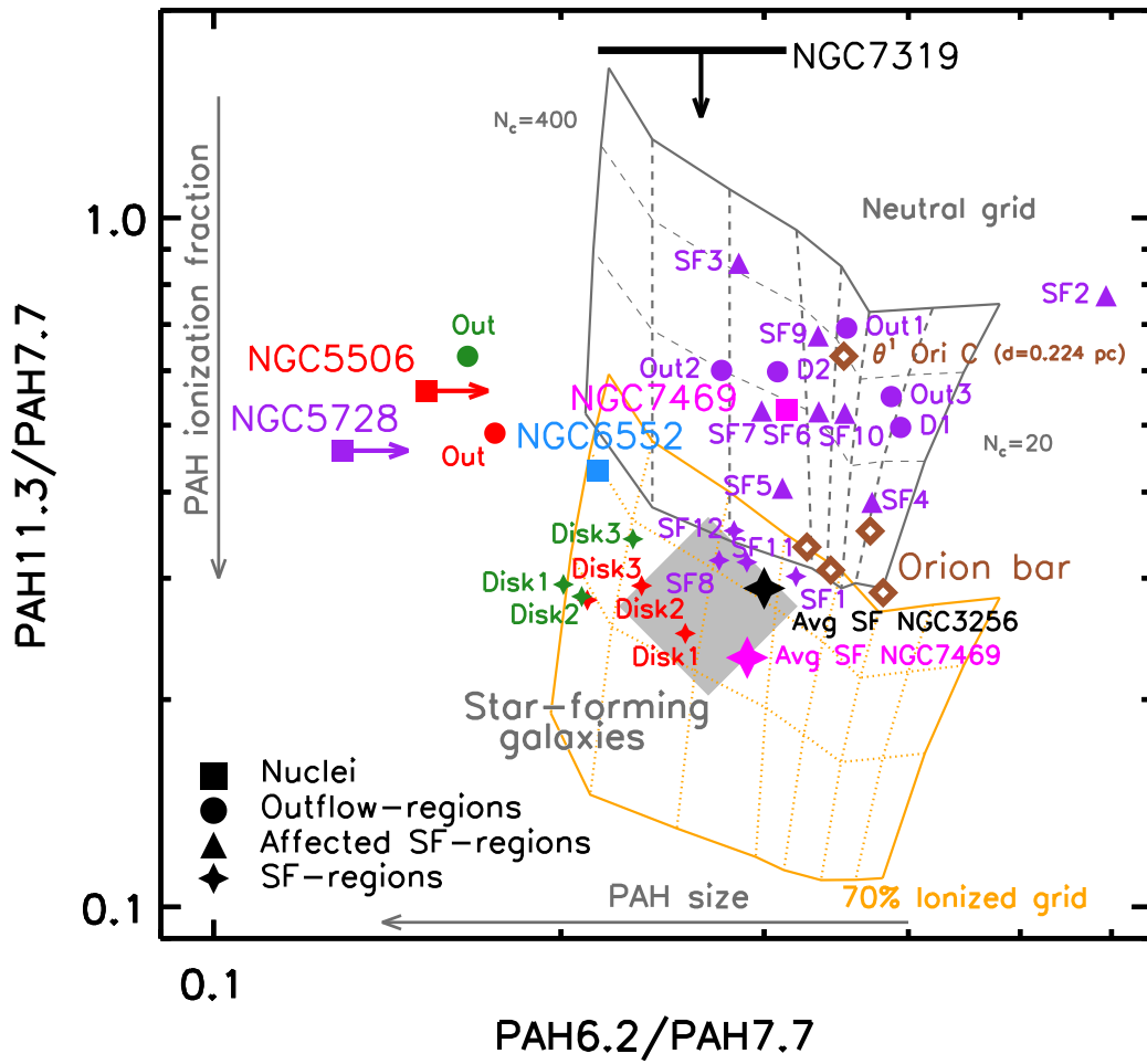
Fig. A.4. Same as Fig. 5, but including all the individual regions. In Tables A.1, A.2, and A.3 we list the measured PAH fluxes.
