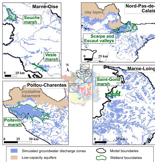
Fig. 4. Comparison between simulated groundwater discharge zones (blue) and RAMSAR-Natura 2000 wetlands (green) location. Areas with low-capacity surface aquifers are excluded from this study (light brown color). (For interpretation of the references to color in this figure legend, the reader is referred to the web version of this article.)
