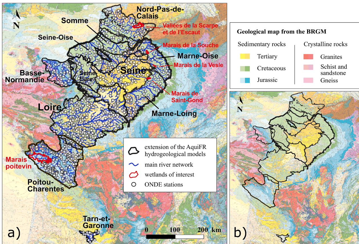
Fig. 1. a) Map of the spatially-distributed groundwater models within the AquifR platform. Simulated rivers predefined in the models are illustrated by blue lines. White dots represent ONDE stations (French observation network of river intermittence). Red polygons delimit wetlands of interest. b) Geological units with a simplified legend (BRGM, 2008). (For interpretation of the references to color in this figure legend, the reader is referred to the web version of this article.)
