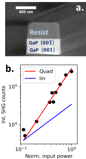
Fig.1.a. Vertical orientation patterned gallium phosphide (VOP-GaP) waveguide. b. Quadratic evolution of the SHG signal's power as a function of the input power.
