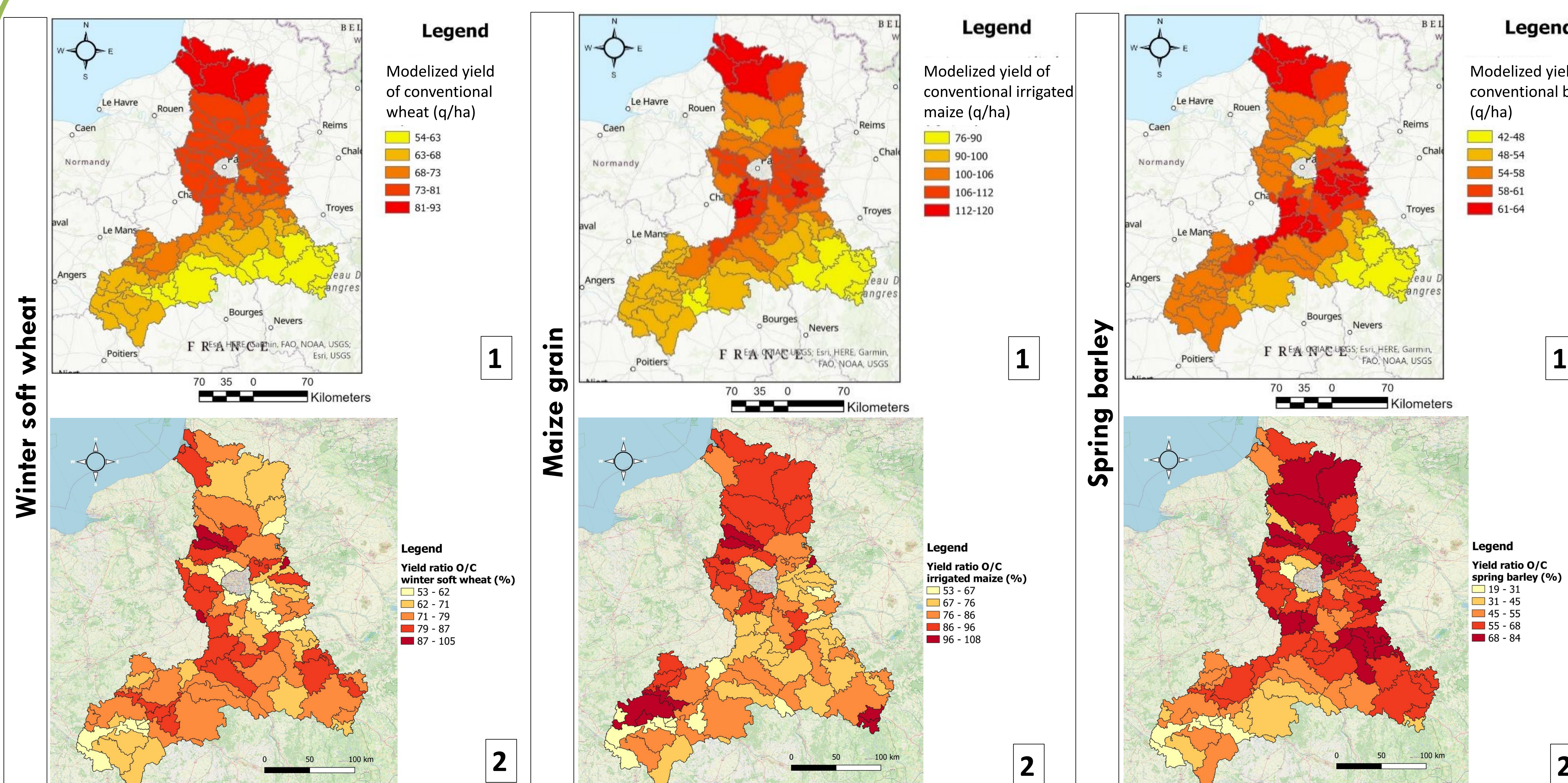
Figure 4. Spatial distribution of estimated yields (quintals/ha) at ASR scale for wheat, maize and barley in conventional farming (1) and the yield ratio organic/conventional (O/C) farming (2)
