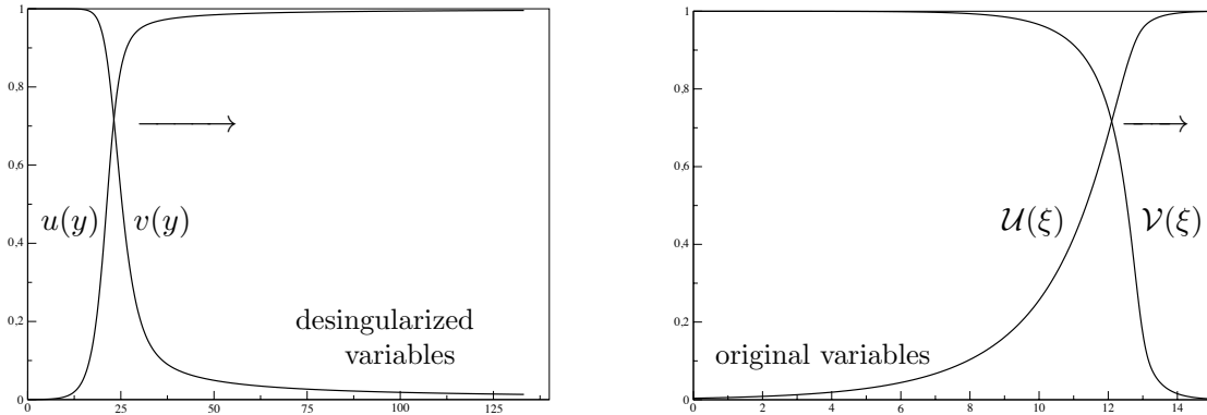
FIGURE 3. The profile of the same propagation front is represented in the desingularized variables (left) and in the original variables (right). The values of the parameters are d = 2 , r = 5 , and c = 0.5 . Note that 1 - u(y) and v(y) converge slowly to zero as y \rightarrow +\infty , in agreement with (2.27), whereas 1 - \mathcal{U}(\xi) and \mathcal{V}(\xi) decay exponentially and may even exhibit a sharp edge when c is small enough. In contrast, the behavior near -\infty is identical in both sets of variables, which is not obvious here because the horizontal scales are very different.
