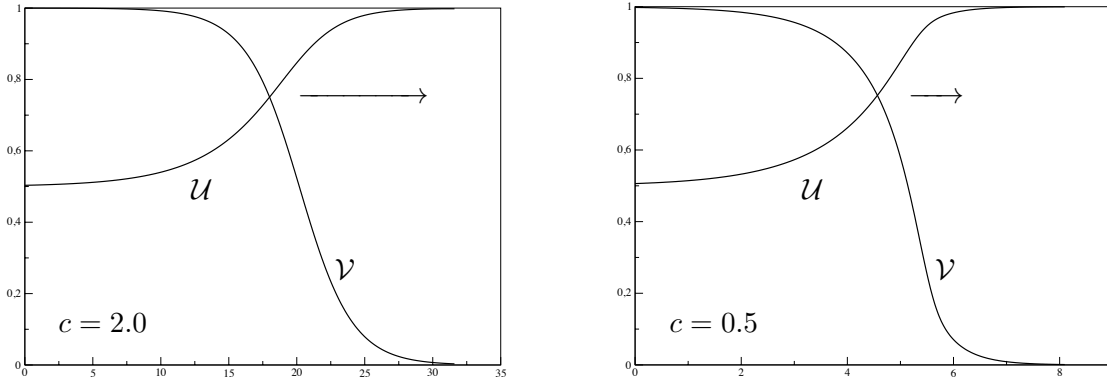
FIGURE 2. The profile (\mathcal{U}, \mathcal{V}) of the front describing heterogeneous invasion is represented for d = 0.5 , r = 1 , and the same values of c as in Fig. 1. Here again the front profile becomes sharper when c is decreased (note that the horizontal scales are different in both pictures), but that phenomenon is less evident than for d = 2 .
