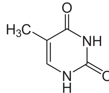
Thymine (ADN)
