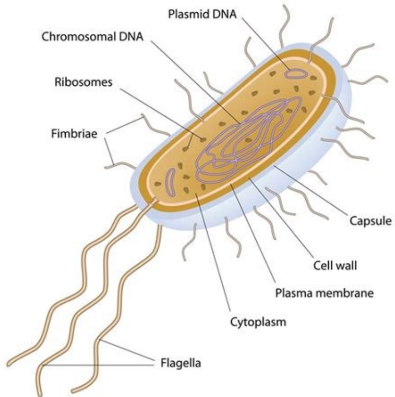
Procaryote
