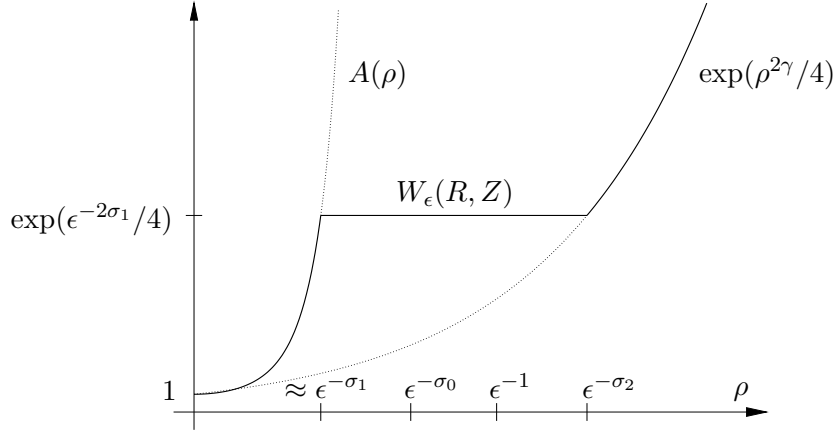
Figure 2: When \epsilon > 0 is small, the weight W_\epsilon(R, Z) entering the energy functional (2.34) is close to a piecewise smooth radially symmetric function, which satisfies W_\epsilon \approx A(\rho) := (4/\rho^2)(e^{\rho^2/4} - 1) in the inner region where \rho := (R^2 + Z^2)^{1/2} \lesssim \epsilon^{-\sigma_1} . When W_\epsilon reaches the threshold value \exp(\epsilon^{-2\sigma_1}/4) , the weight is taken approximately constant until \rho = \epsilon^{-\sigma_2} , and outside that region we set W_\epsilon \approx \exp(\rho^{2\gamma}/4) with \gamma = \sigma_1/\sigma_2 . The dashed lines reflect the fact that \exp(\rho^{2\gamma}/4) \lesssim W_\epsilon \lesssim A(\rho) where the implicit constants do not depend on the parameter \epsilon . The intermediate scales \epsilon^{-\sigma_0} , where the truncation (2.28) occurs, and \epsilon^{-1} , which is the distance from the origin to the boundary \partial\Omega_\epsilon , are indicated for completeness.
