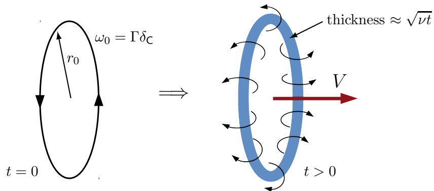
Figure 1: An illustration our main result. Starting from a vortex filament supported on an oriented circle C , the solution of the Navier-Stokes equation evolves into a viscous vortex ring of thickness proportional to \sqrt{\nu t} which moves along the symmetry axis at a speed V given by the Kelvin-Saffman formula (1.5). In the right picture, the vortex lines are circles that fill the solid torus depicted in blue, whereas the black arrows denote the trajectories of the fluid particles.
