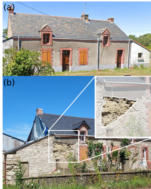
Figure 17. Example of a house before (a) and during (b) the renovation of the external coating showing an unexpected cob part.
