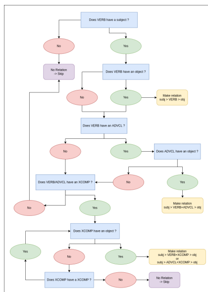
Figure 2: Annotation flowchart.
