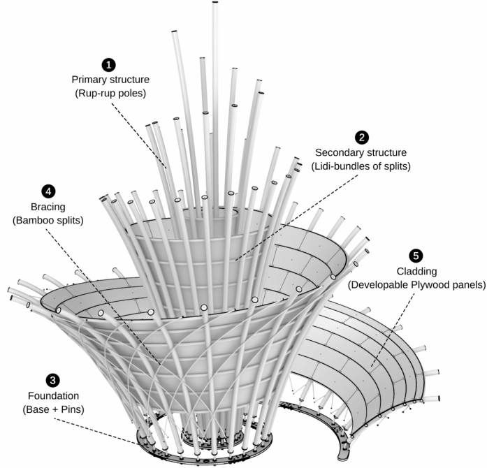
Figure 6: Structural components
