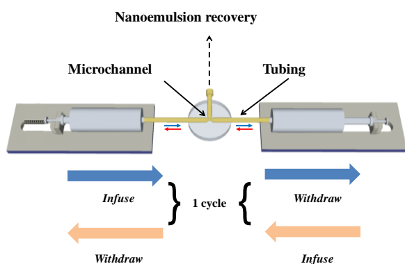
Scheme 1. Schematic illustration of the elongational-flow reactor and mixer.
