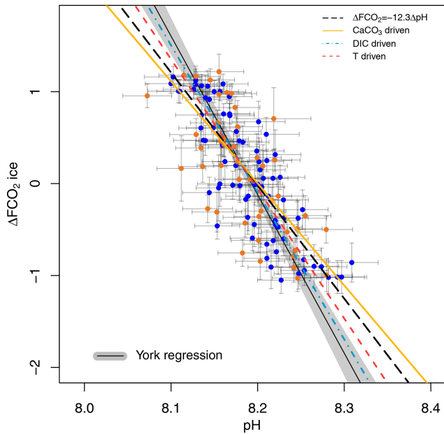
Figure 4. Ice-core-based \Delta\text{FCO}_2 ( \text{CO}_2 forcing) vs. \delta^{11}\text{B} -based pH for ODP 999 (filled blue circles, this study and published data from Foster, 2008; Henehan et al., 2013; Chalk et al., 2017) and 871 (filled orange circles). The lines show the relationship between \Delta\text{FCO}_2 and pH for the simplified formalism (see Sect. 2) \Delta\text{FCO}_2 = -12.3 \Delta\text{pH} (dashed black line) and when driven by changes in DIC only (dashed-dotted blue line, \Delta F/\Delta\text{pH} = -16 \text{ W m}^{-2} ), \text{CaCO}_3 (yellow line, \Delta F/\Delta\text{pH} = -11.1 \text{ W m}^{-2} ), and temperature T (dashed red, \Delta F/\Delta\text{pH} = -14.1 \text{ W m}^{-2} ). The York regressed line (thin black line and grey shading) falls close to the DIC-driven line (dashed-dotted blue line).
