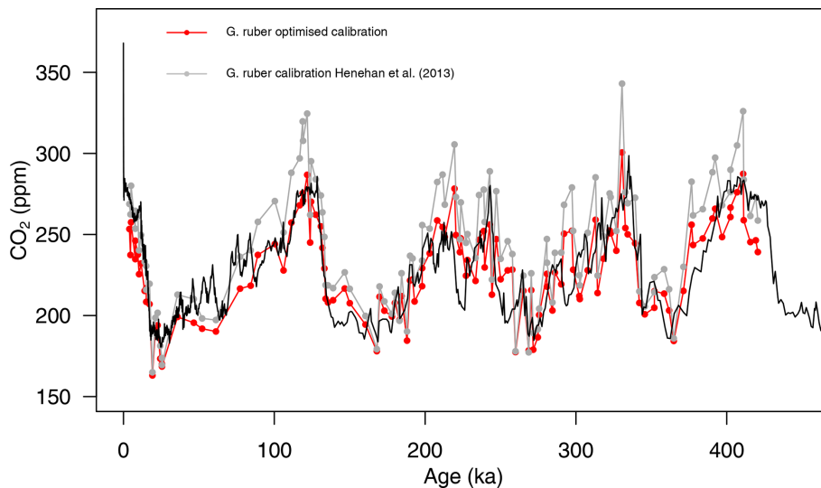
Figure 6. Composite \delta^{11}\text{B} -derived CO 2 from both core sites 999 and 871 using the published \delta^{11}\text{B}_{\text{foram-borate}} calibration (grey points, Henehan et al., 2013) and the optimised calibration (red points). The black line is the Antarctic composite ice core CO 2 record (Bereiter et al., 2015).
