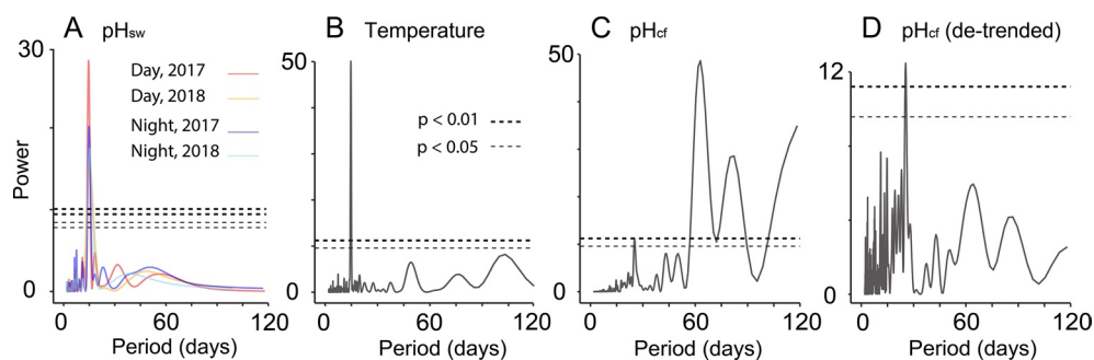
Figure 5. The amplitude of the reef flat \text{pH}_{\text{sw}} and temperature cycle oscillate with a 15 days periodicity: Results of spectral analysis of (a) day time (12 p.m.–4 p.m.) and night time (2 a.m.) \text{pH}_{\text{sw}} and (b) day time (12 p.m.–4 p.m.) seawater temperature. (c) No similar periodicity was found in time series of LA-MC-ICP-MS \delta^{11}\text{B} derived \text{pH}_{\text{cf}} or (d) the similar de-trended (differenced) time series. Confidence lines are indicated as thick ( p < 0.01 ) and thin ( p < 0.05 ) dashed lines whereas in (a) confidence lines of day and night 2017 overlap at power = 10.08 ( p < 0.01 ) and power = 8.44 ( p < 0.05 ), as well as the confidence lines of day and night 2018 at power = 9.44 ( p < 0.01 ) and power = 7.81 ( p < 0.05 ).
