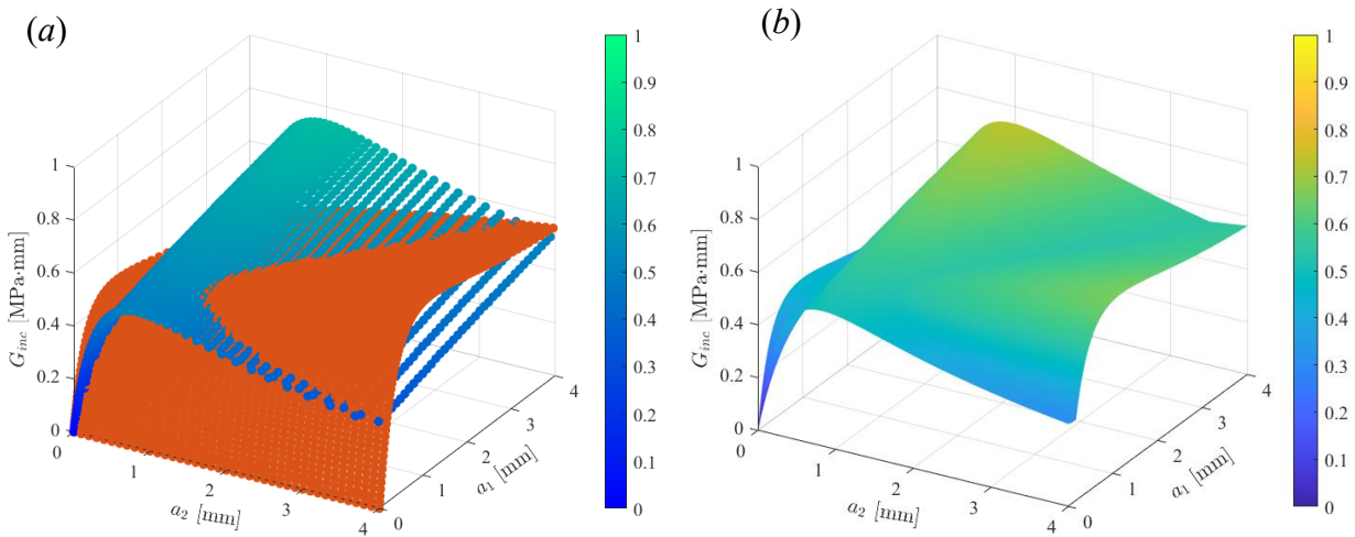
Fig. 7 Geometry characterized by e = 20 mm and \rho = 2 mm: (a) blue/red IERR function for a fixed bottom/top crack, considering nodes unbuttoning along the top/bottom crack path; (b) G_{inc}(a_1, a_2) function obtained taking into account the maximum IERR value for each (a_1, a_2) .
