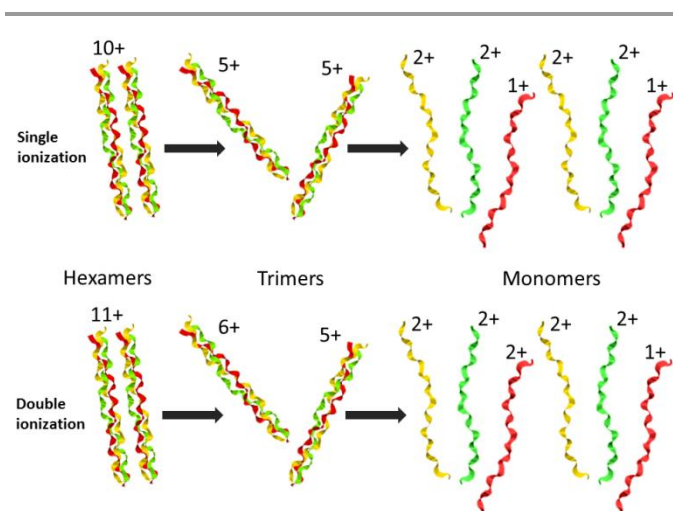
Scheme 1. Dissociation of collagen peptide hexamers after X-ray photoabsorption, single or double ionization and vibrational energy redistribution. The charges of hexamers, trimers and monomers expected from a statistical distribution are indicated.
