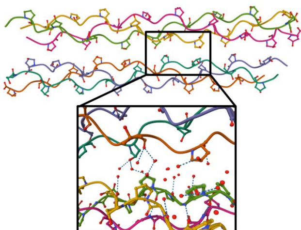
Figure 4. Crystal structure of the (\text{GPO})_9 collagen mimetic peptide hexamer (PDB 3B0S). Peptide backbones are depicted as lines, and only carbon, oxygen (in red) and nitrogen atoms (in blue) of hydroxyproline side-chains are shown. Water molecules are not displayed on the top figure, and on the bottom, only oxygen atoms of the water molecules within 5 Å around green highlighted hydroxyprolines are shown. H bonds are indicated by dashes.
