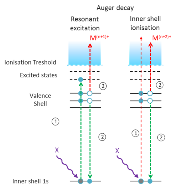
Scheme 2. Electronic processes occurring within a molecular cation M^{n+} after X-ray photoabsorption around atomic K-edges of heavy atoms. Green arrows illustrate resonant transitions leading to excitation or deexcitation, and red arrows depict ejection to the continuum.
