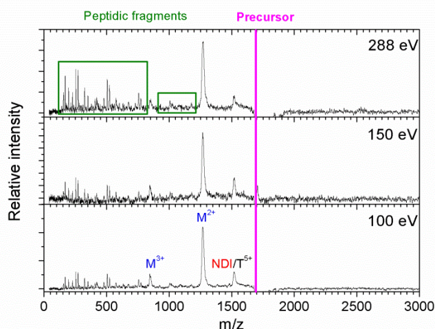
Figure 2. Mass spectra of single-photon absorption products of the collagen mimetic peptide hexamer [(\text{PPG})_{10}_6+9\text{H}]^{9+} (average m/z = 1688 ). NDI, M and T stand for non-dissociative single ionization, monomer and trimer, respectively.
