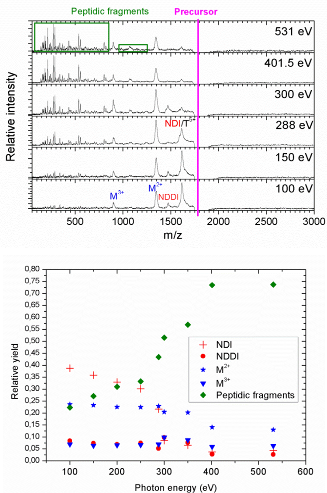
Figure 3. Top: mass spectra of single-photon absorption products of the collagen mimetic peptide hexamer [(\text{POG})_{10}_6+9\text{H}]^{9+} (average m/z = 1795 ). Bottom: relative yield of these products (area under the corresponding peaks normalized to the total yield of product ions) as a function of photon energy. NDI = non-dissociative single ionization, NDDI = non-dissociative double ionization, M^{2+} and M^{3+} are peptide monomers, and "peptidic fragments" is the total fragmentation yield of monomers.
