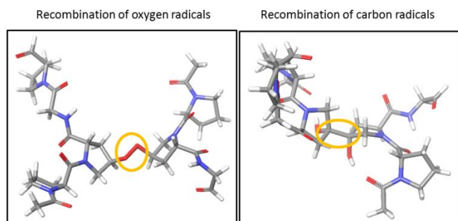
Figure 5. Optimized structures of system A for radicals initially located at oxygens (left) and carbons (right) of the hydroxyproline side chains. The O-O and C-C bonds formed between the hydroxyprolines are encircled. Carbons are depicted in light grey, oxygens in red, nitrogens in blue, hydrogens in white.
