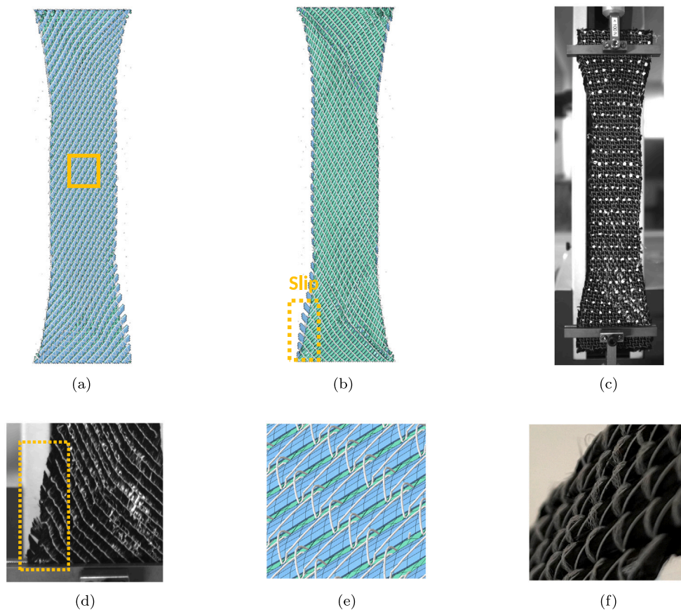
Fig. 18. Results of BET: Deformed configuration of simulated (a, warp yarn, and b, weft yarn) and experimental BET (c, warp yarn); (d) zoom-in view of the experimental edge revealing the occurrence of slips; zoom-in view of the simulated (e) and experimental (f) central shear zones with the presence of both under-tension and bent stitches.
