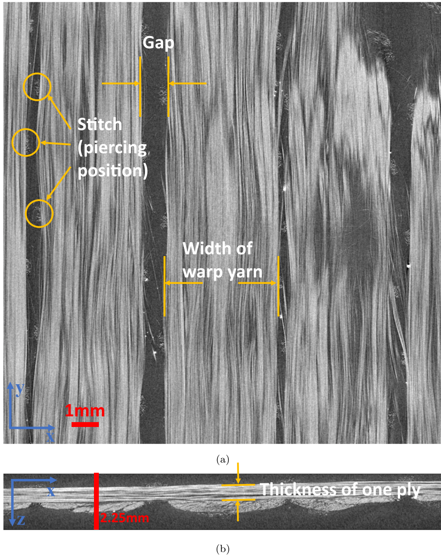
Fig. 3. Measurements of geometrical parameters on tomography results: (a) orthogonal view of a warp yarn ply in the (X, Y) plane, (b) cross-sectional view of the fabric in the (X, Z) plane.
