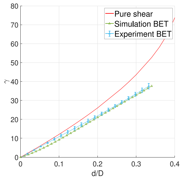
Fig. 20. Comparison of experimental and simulated effective shear angles in BET with theoretical shear angle in pure shear tests, without slippage. Error bars for five experiments.
