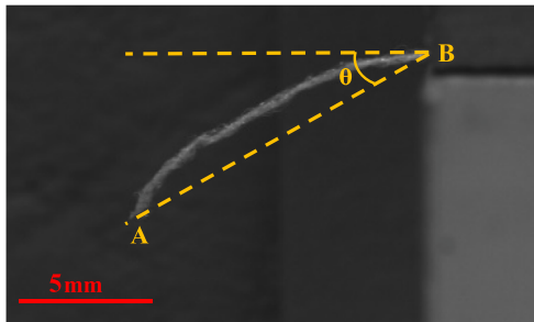
Fig. 11. Single stitch cantilever test.
