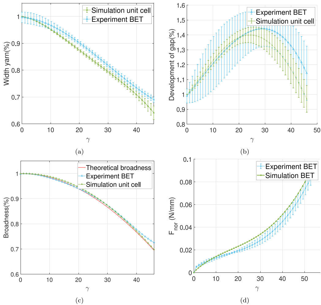
Fig. 21. Comparison between simulation results and experimental tests: (a) Width of yarn vs. shear angle; (b) Development of gap vs. shear angle; (c) Broadness vs. shear angle; (d) shear force vs. shear angle. Error bars for five experiments.
