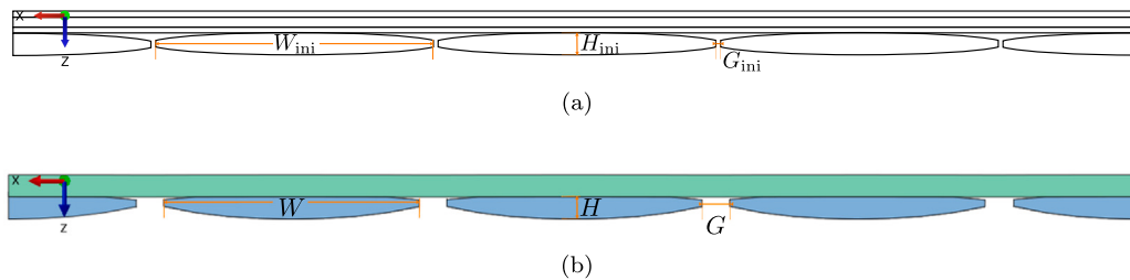
Fig. 4. Cross-sections of the Bi-NCF geometrical model (a) before and (b) after the stitch pre-tension step.
