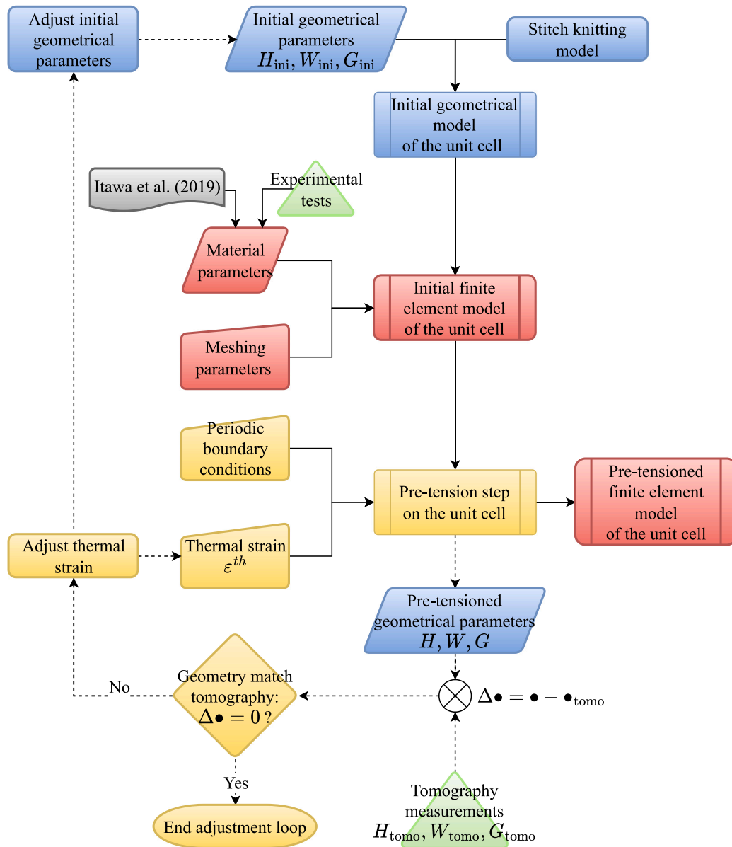
Fig. 13. Flow chart of FE mesoscopic modeling, including the adjustment loop of thermal strain and initial geometrical parameters, represented by dotted-line connectors.
