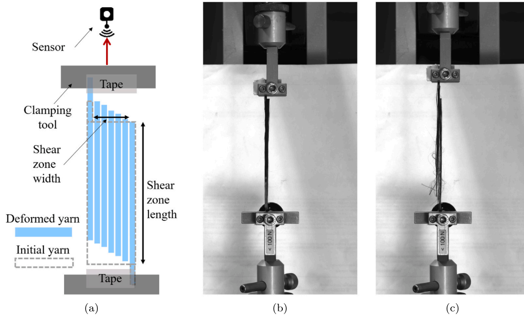
Fig. 8. Longitudinal shear test on a single yarn: (a) Schematic illustration (b) Initial configuration (c) Sample after decohesion of the sample.
