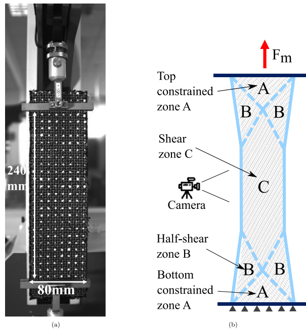
Fig. 17. Bias Extension Test (a) Initial configuration with sample dimensions 240 mm × 80 mm (b) Theoretical solution of BET with zones A (no-shear), B (half shear) and C (maximum shear).
