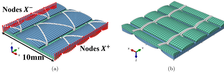
Fig. 12. Finite element representative unit cell of Bi-NCF (a) upper side, warp yarn with zig-zag stitch (b) lower side, weft yarn with looped stitch.
