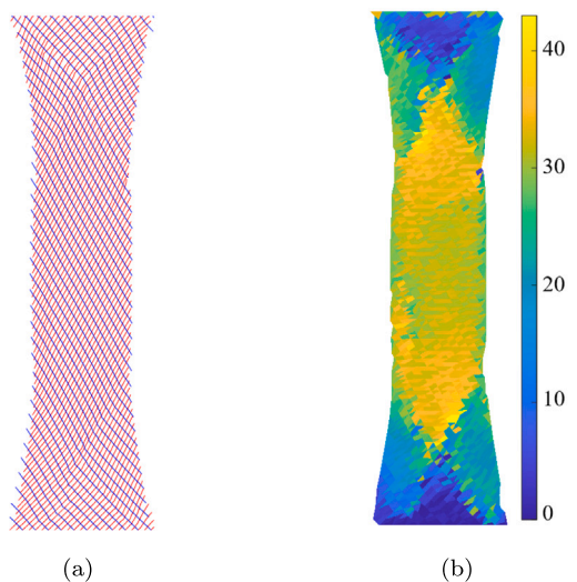
Fig. 19. Calculation of effective shear angle (in degree) in FEM results; (a) Yarn orientation of weft yarn (red) and warp yarn (blue); (b) Shear angle between the two directions, in degree.
