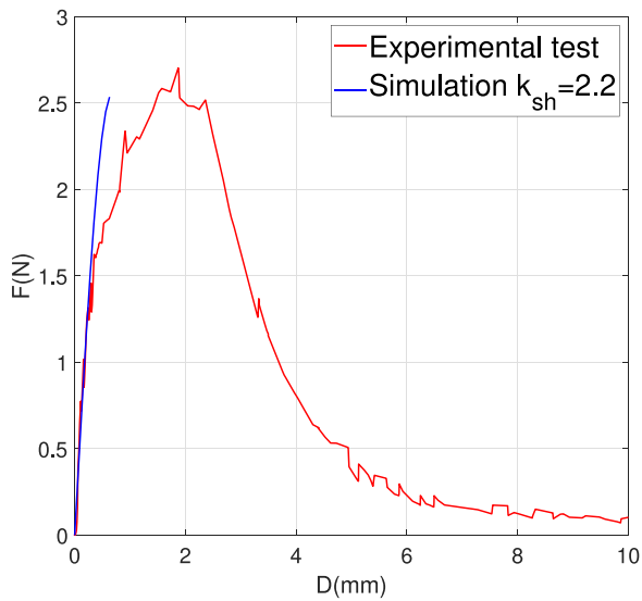
Fig. 9. Longitudinal shear test on a single yarn: force vs. cross-head displacement.
