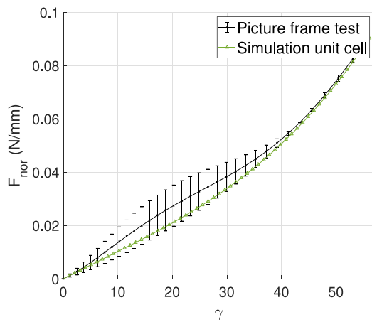
Fig. 15. Normalized shear force of experimental PFT and unit cell shear simulation. Error bars for three tests.
