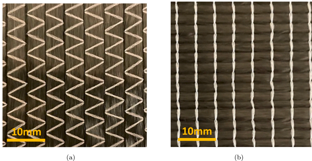
Fig. 1. Bi-NCF (a) Warp yarn view with a zig-zag stitch pattern (b) Weft yarn view with a looped stitch pattern.
