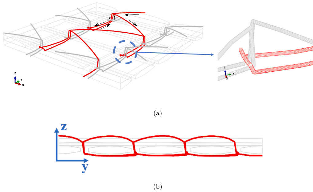
Fig. 5. Tricot stitch model of Bi-NCF. (a) One loop of stitch (red) on a 10 mm \times 10 mm model with a zoomed-in view of its loop connection position. (b) Sectional view ((Y, Z) plane) of the stitch model in the initial configuration (before pre-tension step).
