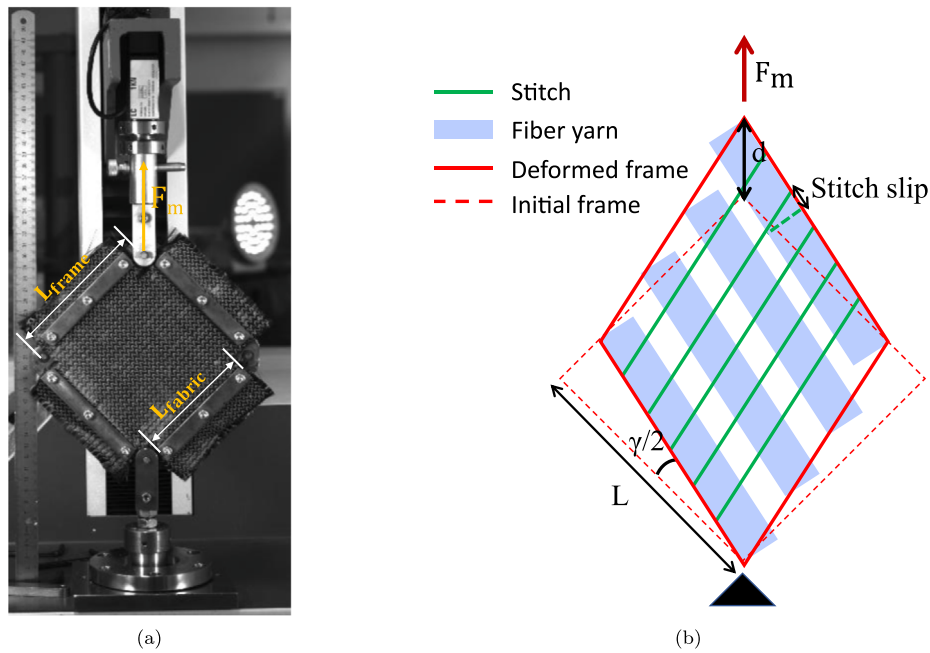
Fig. 14. Picture Frame Test on Bi-NCF (a) Initial configuration on experiments (b) schematic representation of Bi-NCF inside the PFT.
