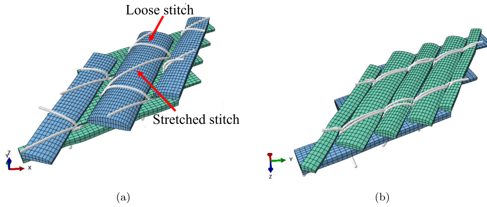
Fig. 16. Deformed configuration of unit-cell under pure shear test (a) upper side, warp yarn with zig-zag stitch (b) lower side, weft yarn with looped stitch.
