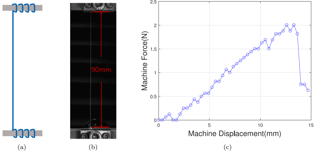
Fig. 10. Tensile test on a piece of stitch (a) Schematic (b) Experimental test initial configuration (c) Force vs. cross-head displacement.
