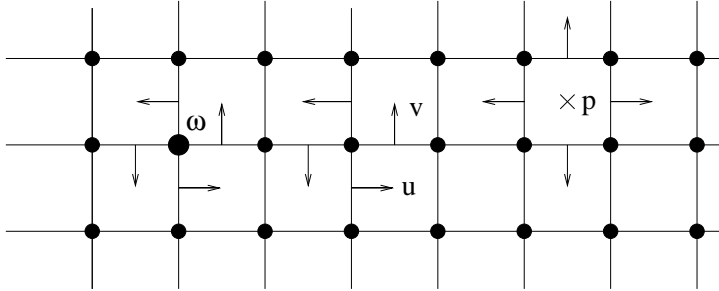
FIG. 1 – The HaWAY scheme on a cartesian mesh.
