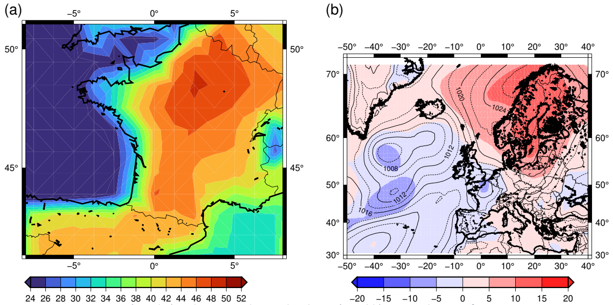
Figure 7: TX over France (panel a) and SLP over the North Atlantic (panel b) on 27 July 2077, for CMCC-ESM2, in SSP2-4.5 (r1i1p1f1). TX (panel a) is expressed in °C. SLP is expressed in hPa (isolines in panel b). Colors in panel (b) correspond to anomalies of SLP (in hPa) with respect to the summer average.
