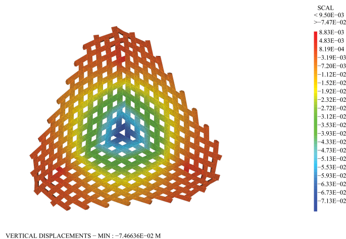
Figure 17: vertical displacement under dead load
