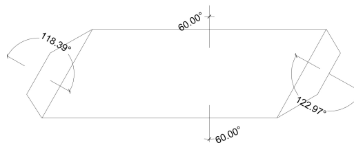
Figure 18: voussoir typology with opposite long edge constant angle and variable small edges angles.
