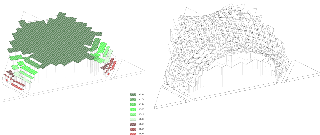
Figure 21: (a) timber formwork with different levels. (b) polystyrene formwork
