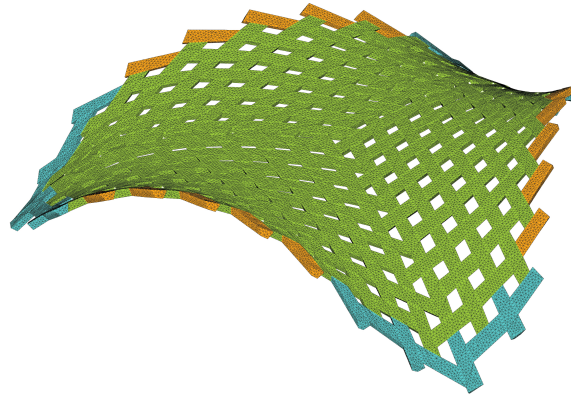
Figure 14: mesh visualization of the structural model
