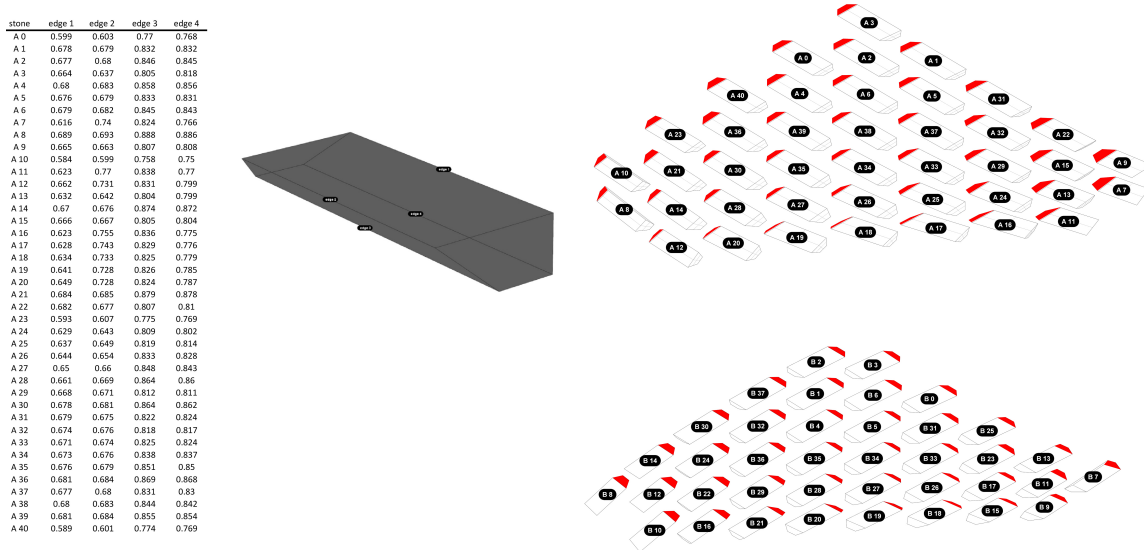
Figure 20: (left) edges lengths verification. (right) templates for voussoirs orientation
