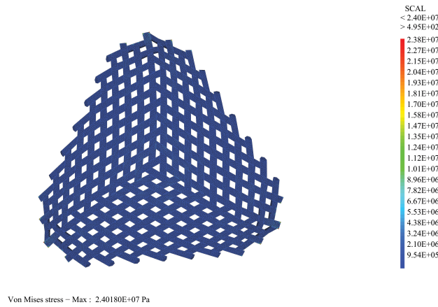
Figure 15: Von Mises stress under dead load
