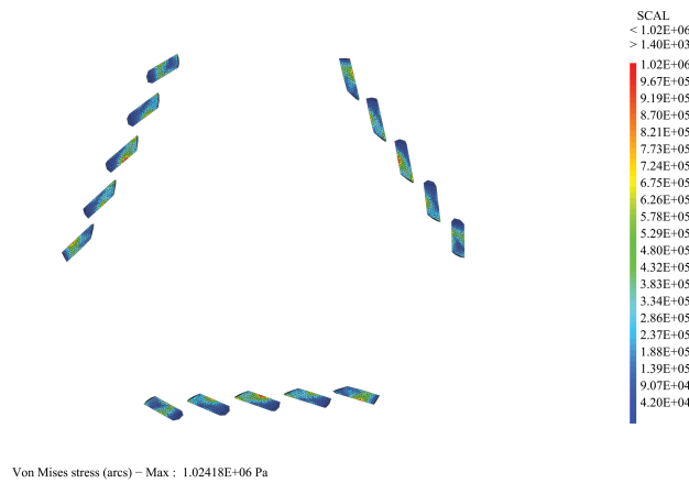
Figure 16: isolated edge voussoirs Von Mises stress under dead load
