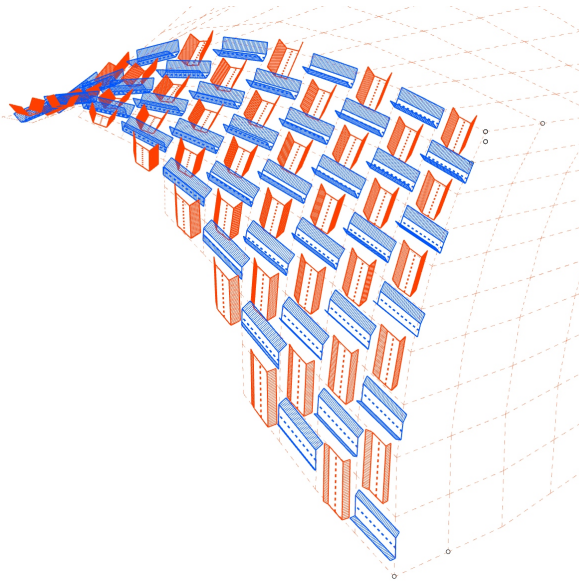
Figure 11: ashlars' long edge planes for both networks
