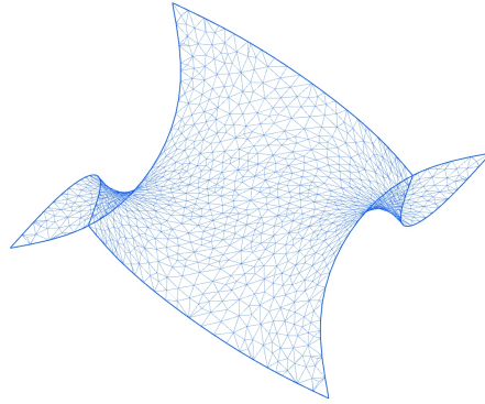
Figure 2 : Mesh representation of the considered gyroid domain
