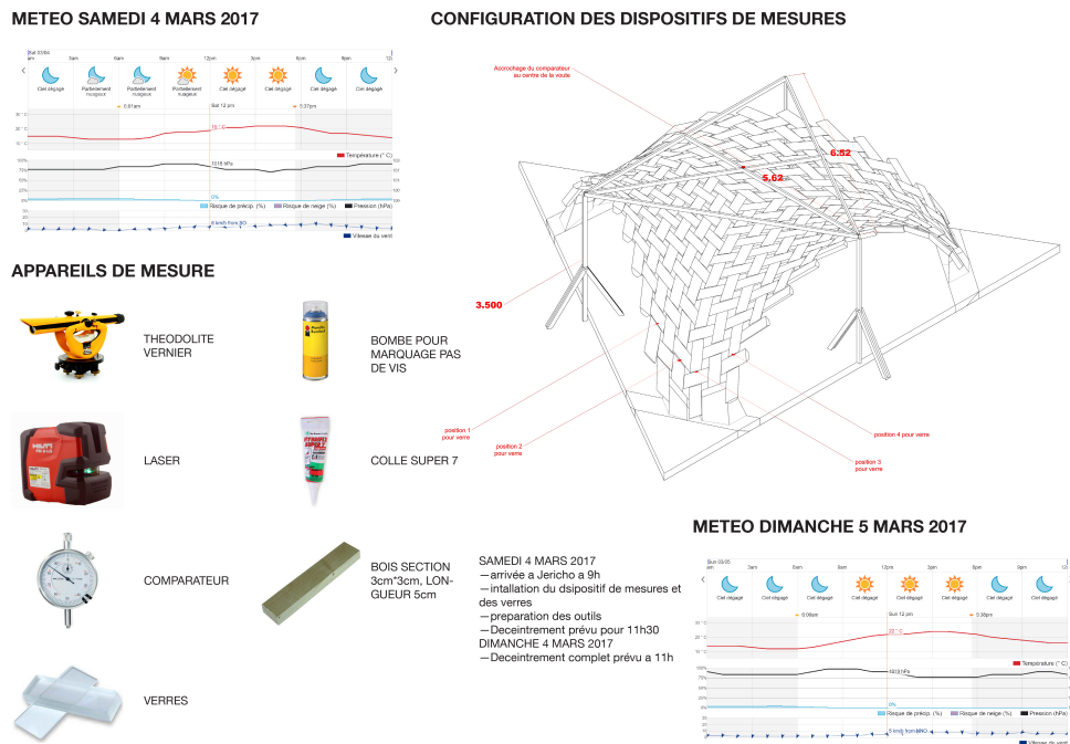
Figure 23: testing and monitoring during un-scaffolding
