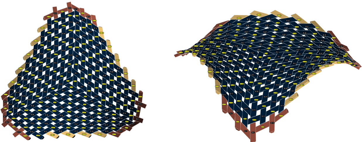
Figure 12: (a) network B ashlars. (b) network A ashlars. (c) both networks.
