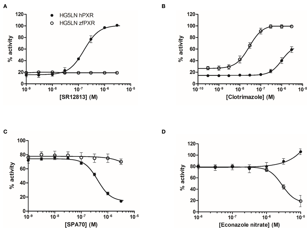
FIGURE 1 | Transcriptional activity of hPXR and zfPXR in response to reference chemicals SR 12813 (A), clotrimazole (B), SPA 70 (C), and econazole nitrate (D). Results are expressed as a percentage of the maximum luciferase activity induced by 3 \mu M SR 12813 (HG5LN-hPXR) or 1 \mu M clotrimazole (HG5LN-zfPXR). Error bars represent standard deviations.
