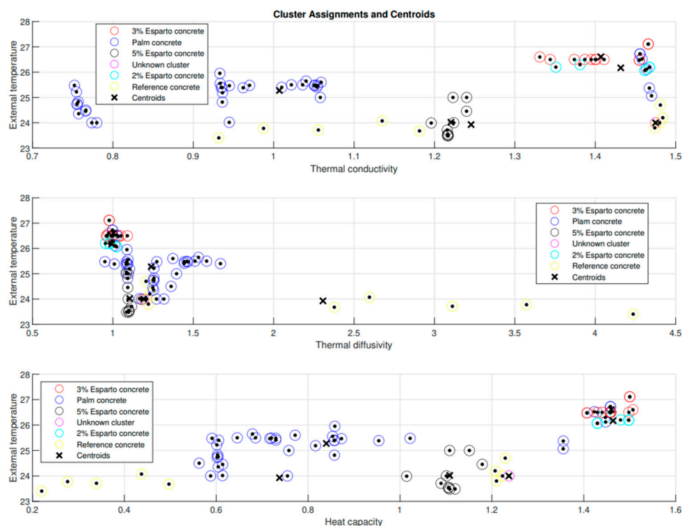
Figure 8. Bio-materials' classification and characterization with six identified clusters.
