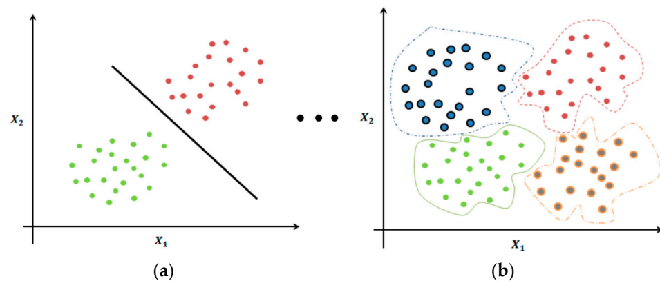
Figure 5. Clustering approach (a) with two identified classes; (b) with multiple identified classes.
