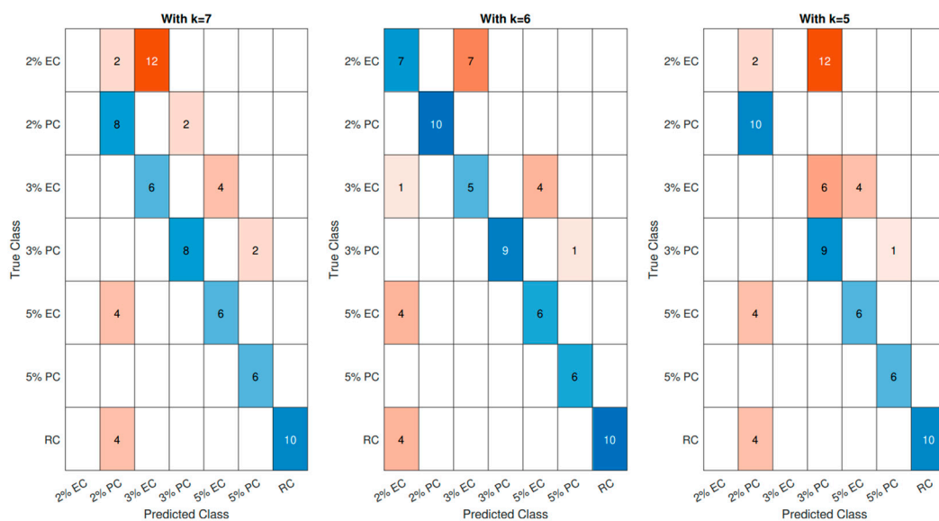
Figure 7. Confusion matrix for different centroid number k = 7, 6 and 5 .
