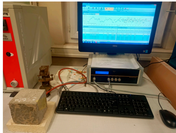
Figure 4. Hot-disk device.
