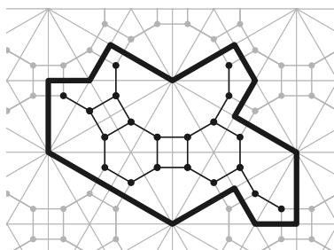
Figure 14: The Turtle tile [SMKGS24] induces a second mildly aperiodic monotile in \Gamma .
