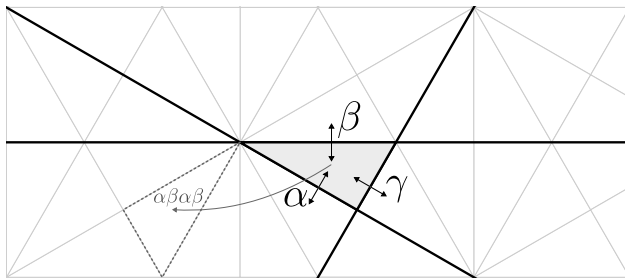
Figure 6: The symmetries of the Semikitegrid.
