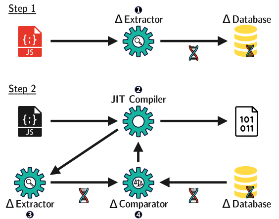
Fig. 2: JITBULL workflow.
