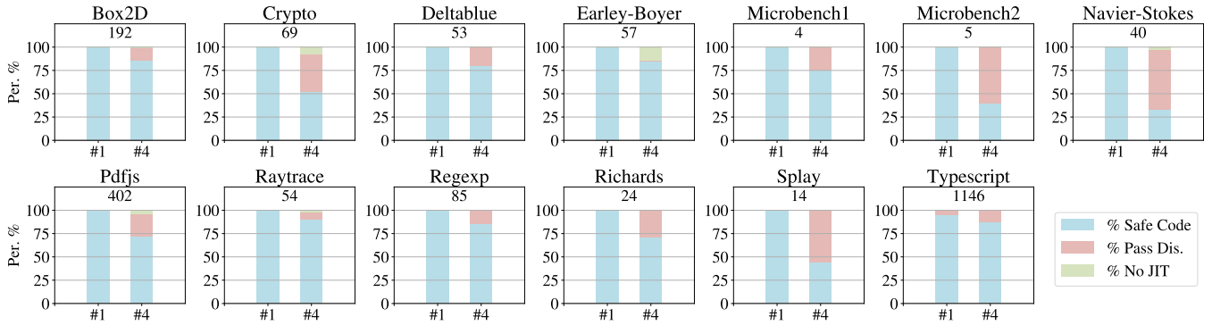
Fig. 4: False positive rates of JITBULL on a set of harmless benchmarks. “#1” and “#4” represent the number of VDCs installed into the JITBULL database (1 versus 4 VDCs respectively).
