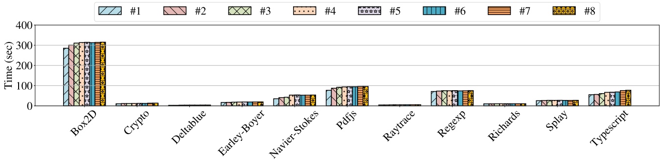
Fig. 6: Scalability evaluation of JITBULL, with various numbers of vulnerabilities in the DB, ranging from #1 to #8.
