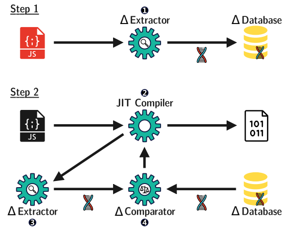
Fig. 2: JITBULL workflow.
