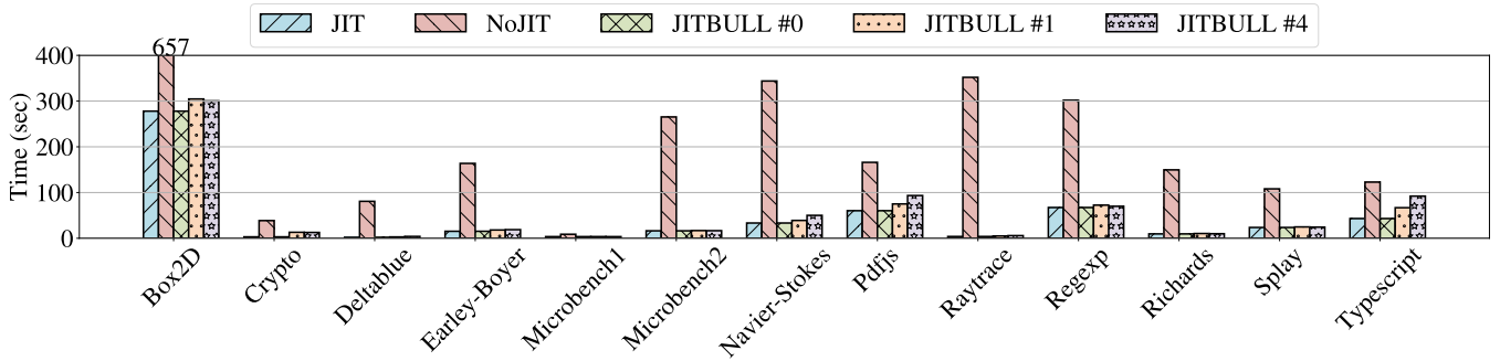
Fig. 5: Execution times for disabled JIT, normal JIT and JITBULL on a set of benchmarks.
