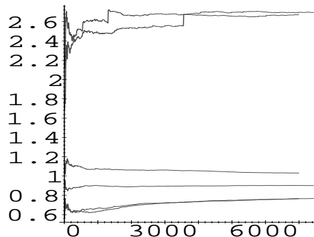
Figure 3: A display of the evolution of search costs and path lengths as a function of the number of strings inserted in standard and hybrid trie structures.
