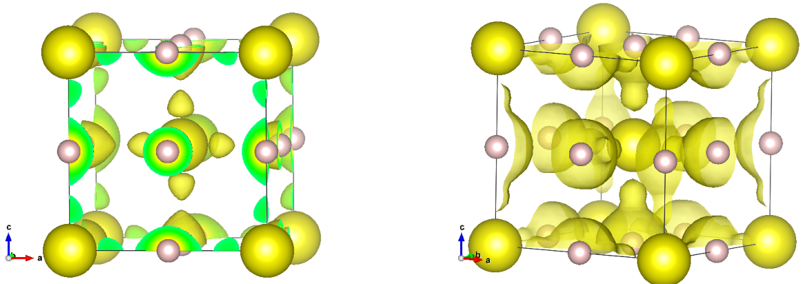
Figure 2: \text{H}_3\text{S} isosurfaces at T=200 K. Left: \rho = 0.002 a.u. Right: \text{ELF} = 0.005 .
