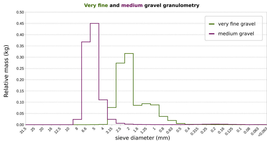
Fig. B.3. Granulometry of very fine gravel and medium gravel . The granulometry was obtained by separating and grouping the sample particle size with a sieve shaker and by weighing the sediment contained in each sieve.
