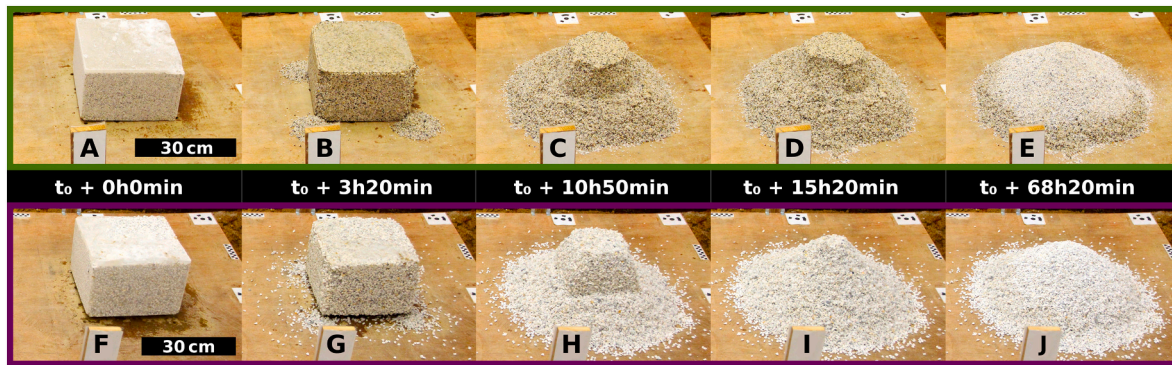
Fig. 5. Degradation of initial frozen block of sediment (EXP6) at different time-steps for both the very fine and medium gravel . We obtain a final conical mound of loose sediment. For time-lapse video see the video supplement.
