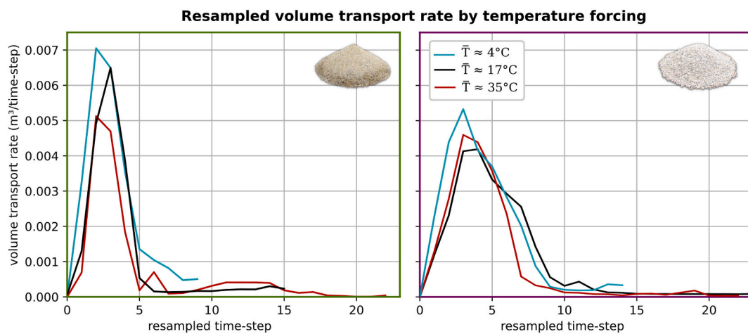
Fig. 10. Volume transport per normalized intervals for very fine (left) and medium gravel (right) during blocks degradation phase for different air temperature forcings. The data from the 4 °C and 17 °C runs have respectively been temporally re-sampled by a factor 1/12 and 1/3 for very fine gravel and by 1/8 and 1/2 for medium gravel to match the 35 °C curves as far as possible. The data was re-sampled by summing over n time steps, where n corresponds to the denominator in the scaling factor. Data from the experimental runs EXP6, EXP8 and EXP9 have been used to create this figure. Small images of molards indicate respective sediment type of the plot.
