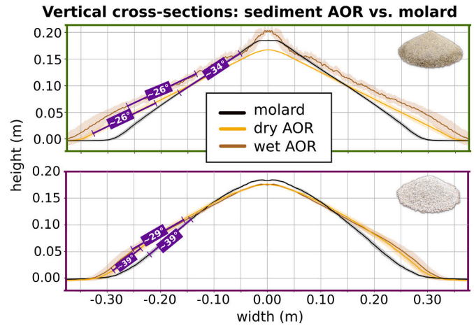
Fig. 8. Rotationally averaged cross-sections of degraded initially frozen block of sediment (molards, EXP6) and lifted box filled with dry or wet sediment for very fine gravel (top) medium gravel (bottom). The shadow represents the standard deviation for the rotationally averaged region. The slope angles are indicated for selected sections marked in purple. The degraded ice-cemented blocks show steeper slope angles in comparison to the corresponding angle of repose. Small images of molards indicate respective sediment type of the plot.
