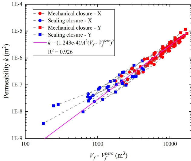
Figure 14. Evolution of the permeability k as a function of the percolation fault volume (the fault volume minus the fault volume at the percolation threshold (V_f - V_f^{perc}) ) for the 6 studied faults, which is fitted by k \approx (B/A^2) \cdot (V_f - V_f^{perc})^2 , where A is the total block area and B = 1.24 \times 10^{-4} is the geometrical prefactor.
