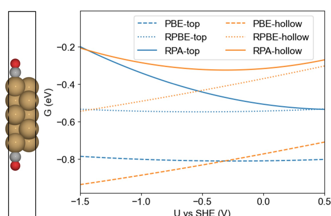
Figure 2 Adsorption energy of CO on Cu(100) as a function of the electrochemical potential at the top (blue) and hollow (orange) adsorption site. RPA predicts CO to be adsorbed at the top site across the whole range of potentials.
