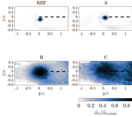
Figure 2. Contours of the normalized averaged axial vorticity \hat{\omega}_x/\hat{\omega}_{x,max} at x/c = 5 .
