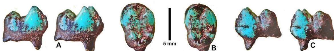
Figure 5. Stereo images of GSN KOM 80'24, left m/2 of Otocyon sp. From Kombat E-900 (fissure 'A'), Otavi Mountainland, Namibia. A – lingual view, B – occlusal view, C – buccal view.
