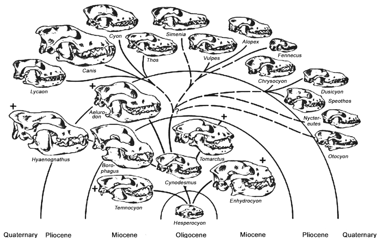
Figure 9. Phylogeny of the Canidae based on Thenius & Hofer (1960). Note the question mark at the base of the Otocyon lineage. « + » signifies the extinction of a lineage.
