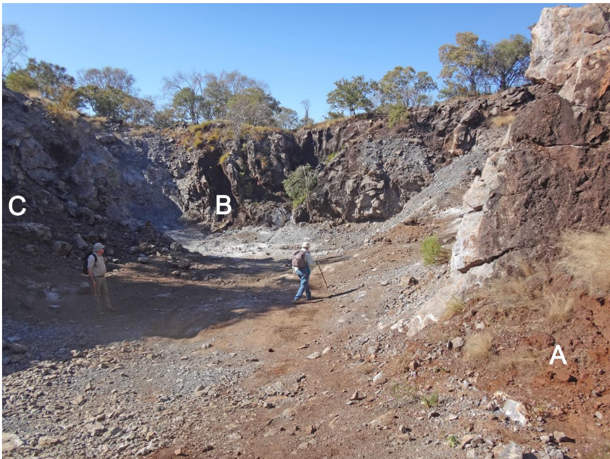
Figure 3. The Kombat E-900 open pit showing the positions of fissures ‘A’, ‘B’ and ‘C’ in dolostones of the Upper Hüttenberg Formation. Fissure ‘B’ is poorly fossiliferous and the ‘C’ fissure contains abundant Middle Stone Age lithic implements and waste flakes.
