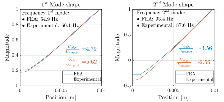
Fig. 9. Comparison between numerical simulations in blue and experimental measurements in red for a prototype with only a leading edge mode
