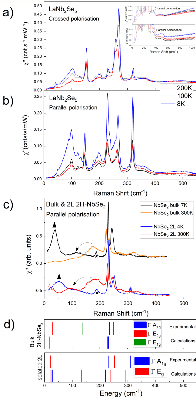
FIG. 3. Temperature dependence of the Raman response of (\text{LaSe})_{1.14}(\text{NbSe}_2)_2 with (ab)-plane crossed (a) and parallel (b) polarisation configurations. Inset: large energy-range electronic Raman response. c) Raman response of bulk 2H- \text{NbSe}_2 and isolated 2L- \text{NbSe}_2 [35] at 300 K and \sim 5 K, in the CDW state. The stars, triangles stands for the Brillouin-zone folded phonons and amplitudons, respectively. The arrows indicate the double phonon modes related to the soft phonon branches of the CDW. (d) Raman active phonons energies from experiments and from theory.
