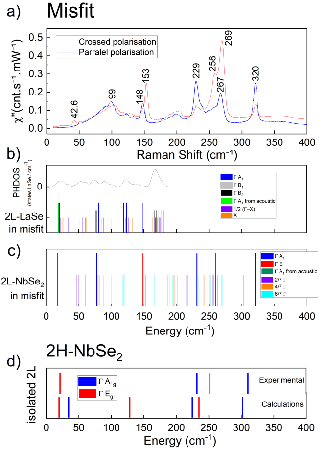
FIG. 4. a) Raman spectra of (\text{LaSe})_{1.14}(\text{NbSe}_2)_2 at 8 K in crossed and parallel polarizations in the (ab)-plane. b) and c) Theoretical calculations of Raman active modes of (\text{LaSe})_{1.14}(\text{NbSe}_2)_2 obtained from those of the two subsystems, namely LaSe (panel b)) and \text{NbSe}_2 (panel c)), electron doped by means of the FET setup. The original modes from \Gamma of the 1 \times 1 cell (long bars) and their subsequent BZ folding (short bars) modes are indicated (Cf. text). Original modes from \Gamma of the 1 \times 1 cell are classified by symmetries. The phonon density of states of LaSe is shown in the upper part of panel b). d) Comparison between experimental [35] and theoretical zone center modes of isolated 2L- \text{NbSe}_2 . Here, the \text{NbSe}_2 lattice parameter is the one in the misfit, namely a=3.437 \text{ \AA} .
