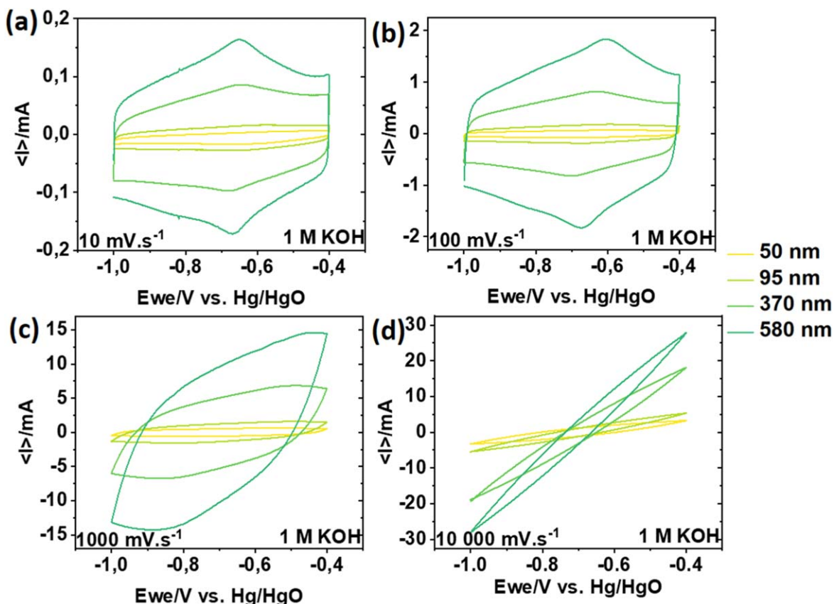
Figure 3 Cyclic voltammograms of vanadium oxynitride thin films between -1 V and -0.4 V vs Hg/HgO in 1 M KOH cycled at (a) 10 \text{mV}\cdot\text{s}^{-1} , (b) 100 \text{mV}\cdot\text{s}^{-1} and (c) 1000 \text{mV}\cdot\text{s}^{-1} and (d) 10\,000 \text{mV}\cdot\text{s}^{-1} .
