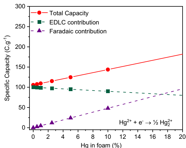
Figure 2. Theoretical capacity (in C\ g^{-1} ) of an electrochemical capacitor using a capacitive material with capacitance = 100\ F\ g^{-1} within a voltage window of 1.0\ V . The contribution of mercury ions undergoing the half-reaction shown in the right-bottom corner increases with the heavy metal cation concentration (purple triangles, dashed line) as does the total capacity (red circles, solid line), while the capacitive (non-faradaic) contribution decreases (green squares, dashed line).
