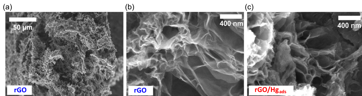
Figure 4. a,b) SEM images of the pure rGO and c) rGO/ \text{Hg}_{\text{ads}} .
