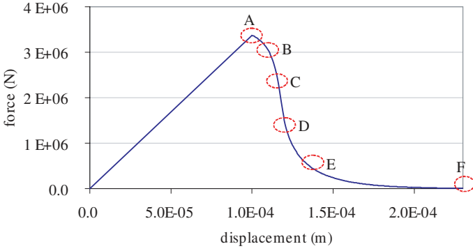
Figure 3: Global response of the bar in traction.
