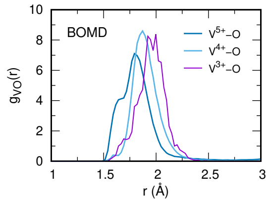
Figure 7: (Colors online) V-O partial pair correlation functions for different oxidation states of vanadium. Upper part: CMD results, lower part: BOMD results.
