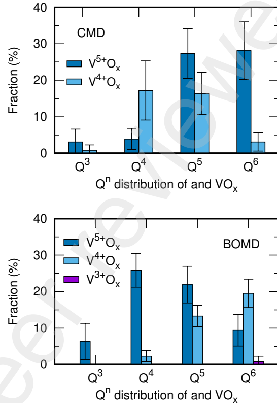
Figure 10: Q n distribution (with n the number of bridging oxygen per polyhedra unit) of VO x (for V 5+ , V 4+ , and V 3+ oxidation states) units describing the network connectivity in glassy VP50.
