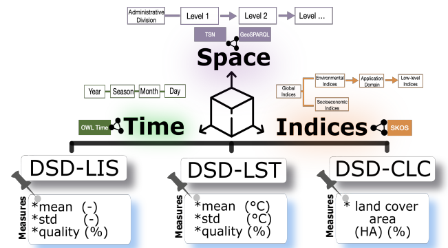
Figure 3. Final DSD design of the three EO-RDF data cubes.
