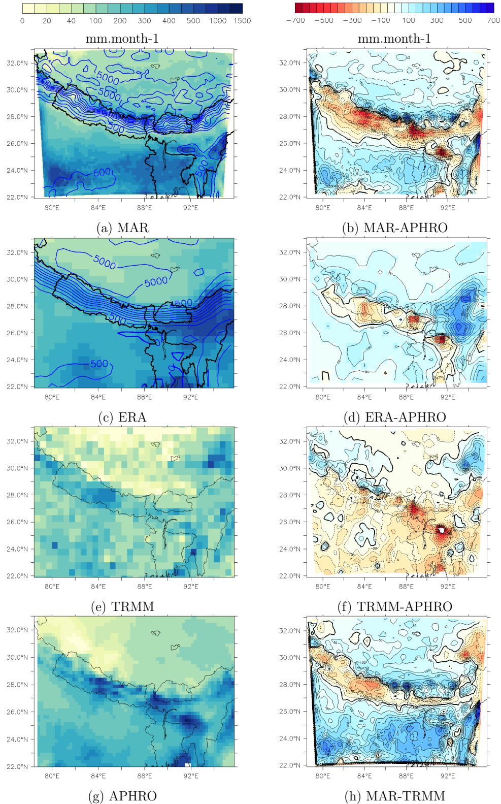
Fig. 3. Monsoon (JJAS) 2001 precipitation (mm month -1 ): (a) simulated with MAR, (c) estimated from ERA-INTERIM, (e) evaluated from TRMM, and (g) observed with APHRODITE network. Figures in the right column correspond to the differences (b) MAR-APHRODITE, (d) ERAINTERIM-APHRODITE, (f) TRMM-APHRODITE, and (h) MAR-TRMM.
