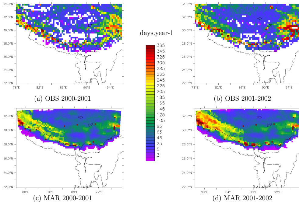
Fig. 6. Snow cover duration: (a) 2000–2001 and (b) 2001–2002 IMS observation (NSIDC, 2004); (c) 2000–2001 and (d) 2001–2002 MAR simulation. Annual values are computed from October to October.
