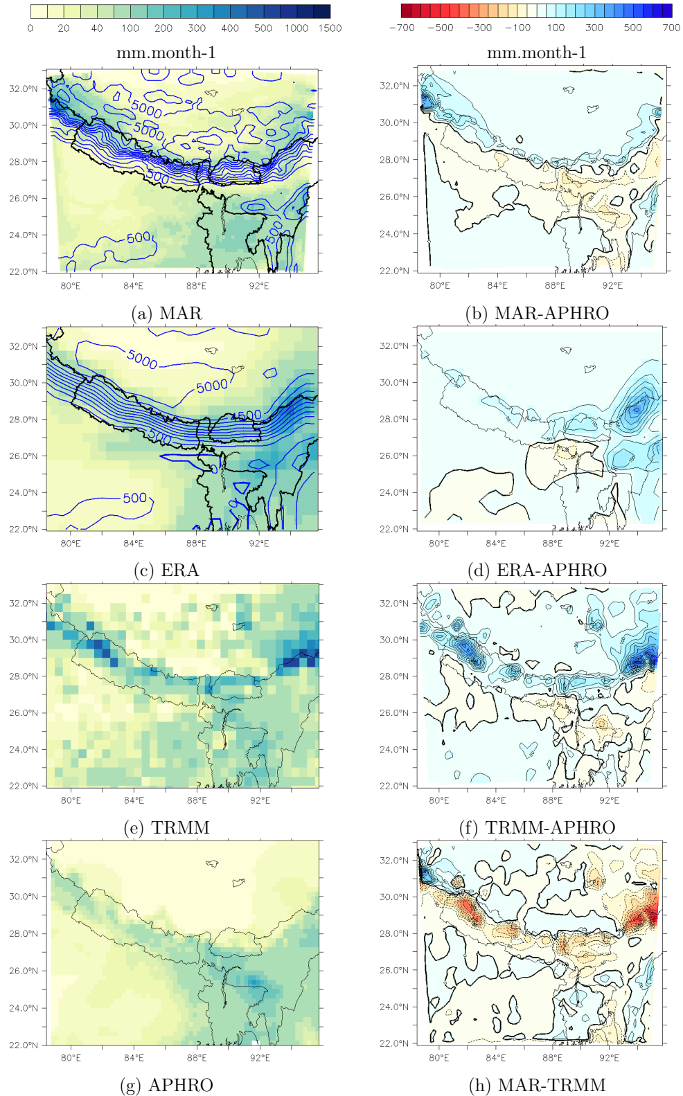
Fig. 4. Extra-monsoon (ONDJFMAM) 2001–2002 precipitation (mm month -1 ): (a) simulated with MAR, (c) estimated from ERA-INTERIM, (e) evaluated from TRMM, and (g) observed with APHRODITE network. Figures in the right column correspond to the differences (b) MAR-APHRODITE, (d) ERA-INTERIM-APHRODITE, (f) TRMM-APHRODITE, and (h) MAR-TRMM.
