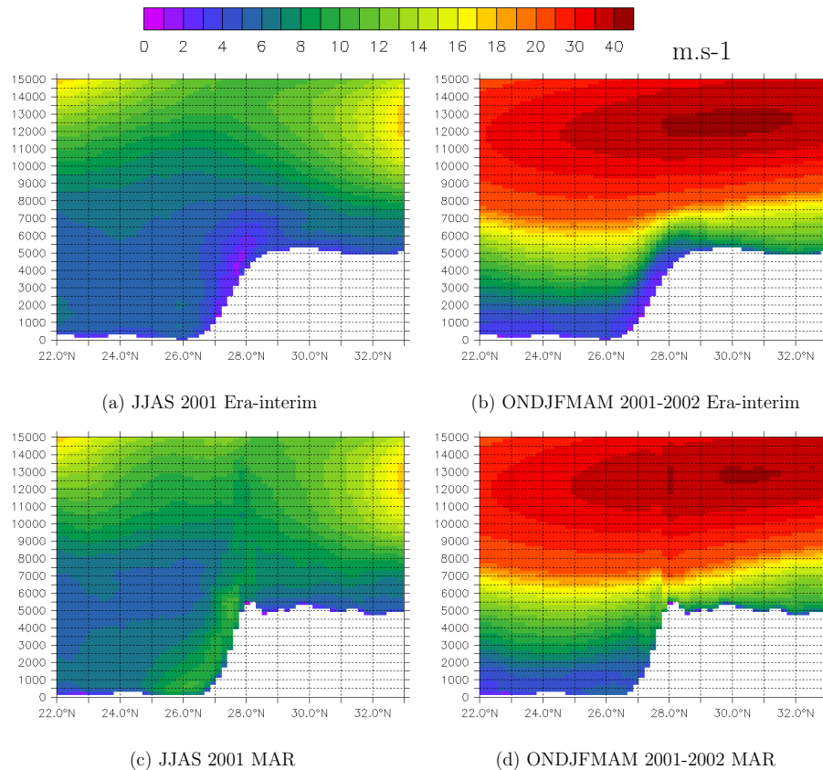
Fig. 2. Wind intensity temporally averaged at the longitude 86^{\circ} E: estimated from the ERA-INTERIM during (a) monsoon (JJAS) 2001, (b) extra-monsoon period (ONDJFMAM) 2001–2002, and simulated with MAR during (c) monsoon (JJAS) 2001 and (d) extra-monsoon period (ONDJFMAM) 2001–2002.
