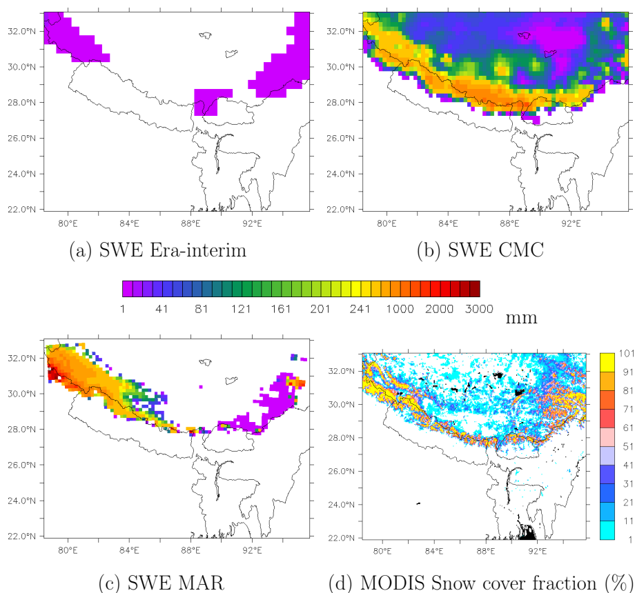
Fig. 5. April 2001 Snow Water Equivalent (mm): (a) estimated from the ERA-INTERIM, (b) evaluated by the Canadian Meteorological Centre (CMC) and (c) simulated with MAR. (d) shows the Snow Cover Extent (SCE) observed with MODIS for the same period.
