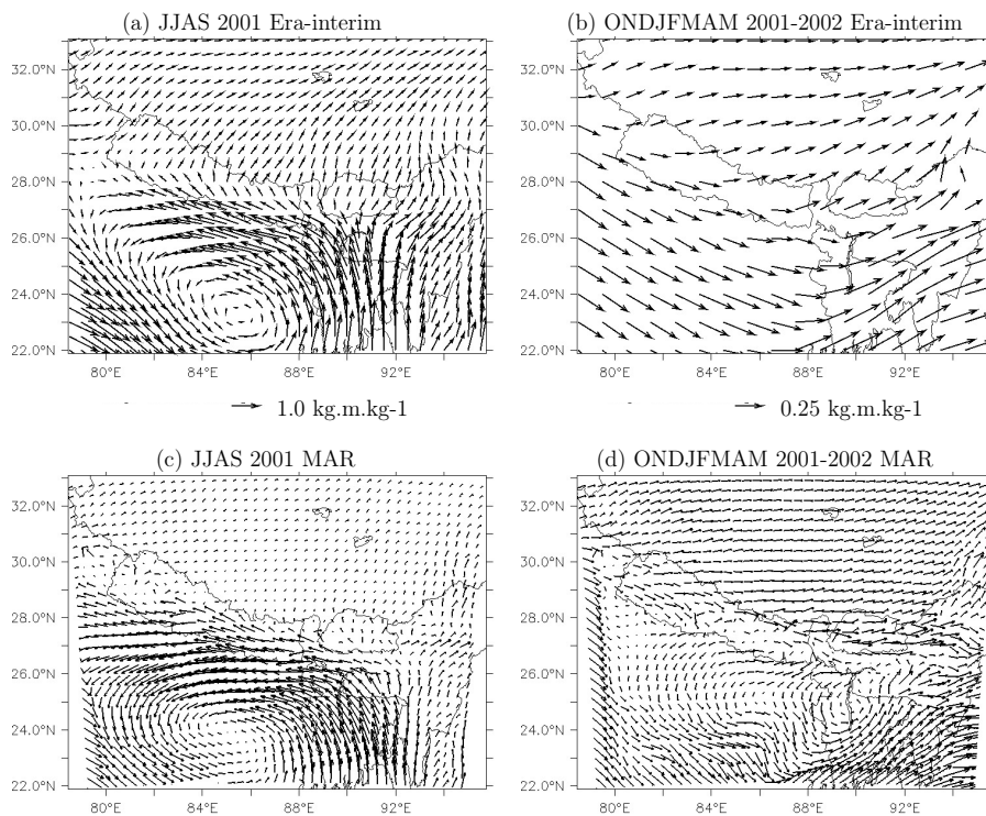
Fig. 1. Moisture flux ( \text{kg m kg}^{-1} \text{ s}^{-1} ) defined as wind velocity multiplied by specific humidity: estimated from the ERA-INTERIM during (a) monsoon (JJAS) 2001, (b) extra-monsoon period (ONDJFMAM) 2001–2002, and simulated with MAR during (c) monsoon (JJAS) 2001 and (d) extra-monsoon period (ONDJFMAM) 2001–2002.
