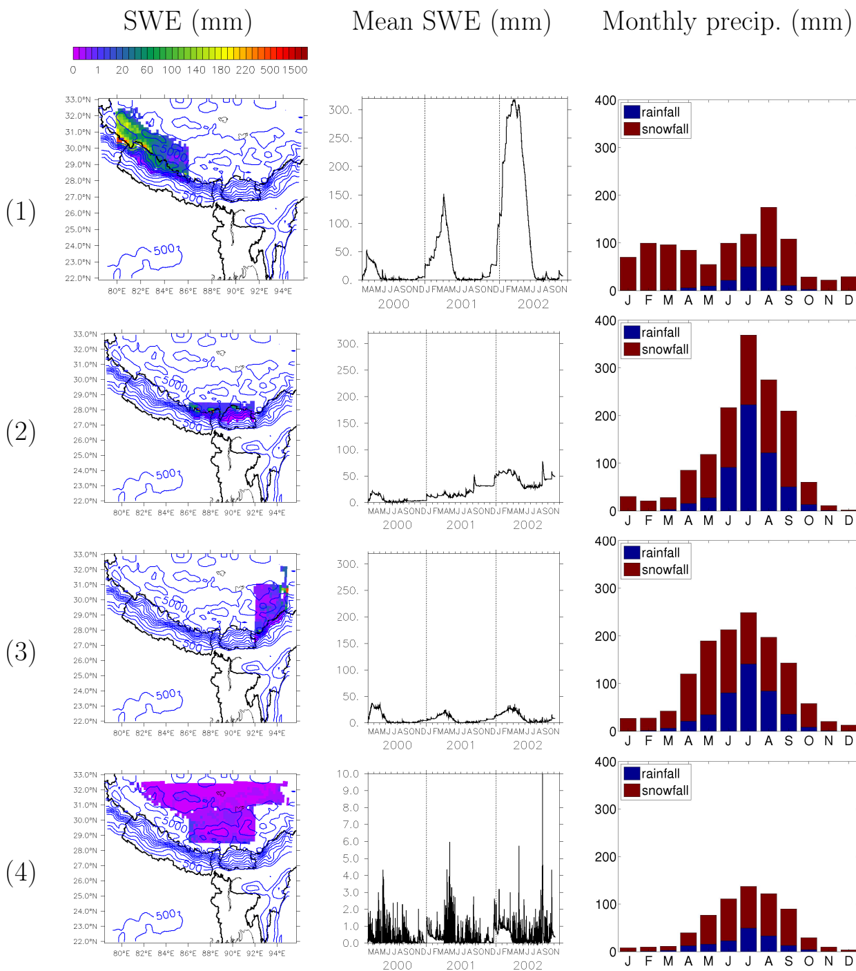
Fig. 8. Snow Water Equivalent (SWE, mm, first column), mean SWE (mm, second column) and annual cycle of precipitation (third column, monthly means of snowfall and rainfall over 2000–2002) for the domain areas coloured in the first column (subsectors numbered from 1 to 4, all altitudes exceed 2500 m a.s.l.).
