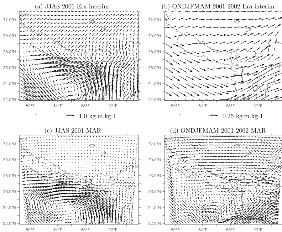
Fig. 1. Moisture flux ( \text{kg m kg}^{-1} \text{s}^{-1} ) defined as wind velocity multiplied by specific humidity: estimated from the ERA-INTERIM during (a) monsoon (JJAS) 2001, (b) extra-monsoon period (ONDJFMAM) 2001–2002, and simulated with MAR during (c) monsoon (JJAS) 2001 and (d) extra-monsoon period (ONDJFMAM) 2001–2002.
