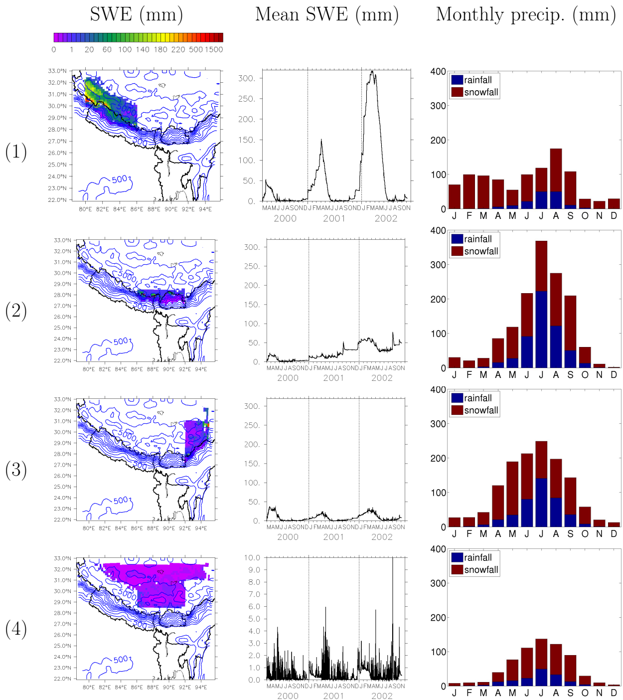
Fig. 8. Snow Water Equivalent (SWE, mm, first column), mean SWE (mm, second column) and annual cycle of precipitation (third column, monthly means of snowfall and rainfall over 2000–2002) for the domain areas coloured in the first column (subsectors numbered from 1 to 4, all altitudes exceed 2500 m a.s.l.).
