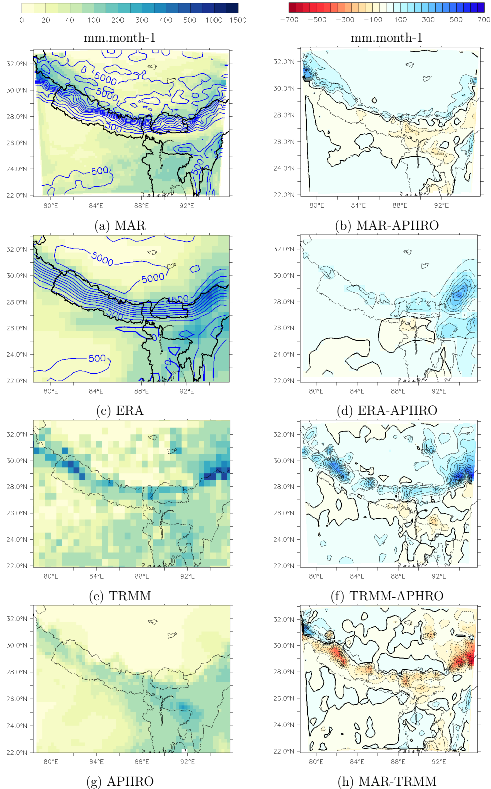
Fig. 4. Extra-monsoon (ONDJFMAM) 2001–2002 precipitation (mm month -1 ): (a) simulated with MAR, (c) estimated from ERA-INTERIM, (e) evaluated from TRMM, and (g) observed with APHRODITE network. Figures in the right column correspond to the differences (b) MAR-APHRODITE, (d) ERA-INTERIM-APHRODITE, (f) TRMM-APHRODITE, and (h) MAR-TRMM.
